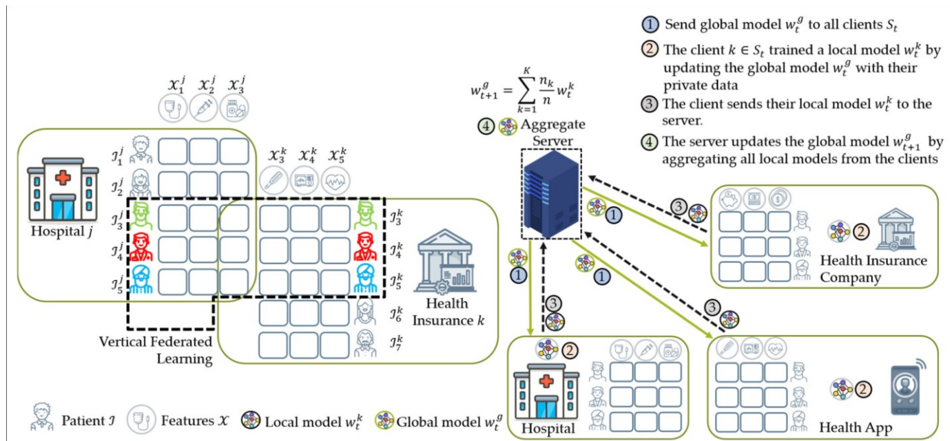
Figure 7. The typical medical data partitions scenario for vertical federated learning (VFL). Each node can be a different medical institution and application. They share the same patients' index I_j = I_k but have different features of medical diagnosis X_j \neq X_k .
