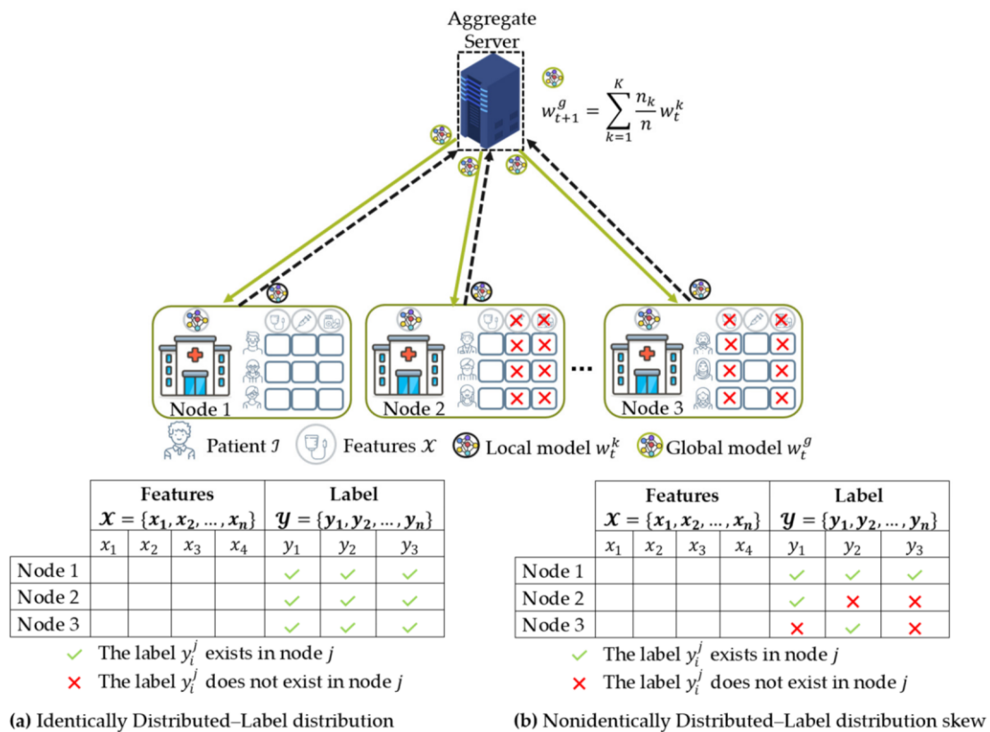
Figure 10. Non-IID from label distribution skew (prior probability shift) characteristic. (a) IID: The distribution of labels Y exists in all nodes; (b) non-IID: the distribution of labels Y varies between different nodes. For instance, node two does not have the labels y_2 and y_3 while node one has all labels.
