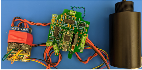
Figure 9: The acoustic modem and the transducer.
