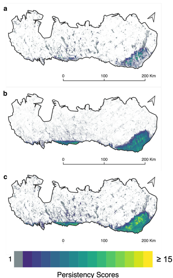
Fig. 9. Heatmap showing the number of times (i.e. persistence scores) each pixel is classified as (a) slush, (b) ponded water and (c) either slush or ponded water over all of the 15-day products produced for the full study period (2013–20).
