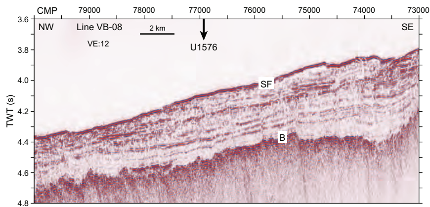
Figure F18. Regional section of Seismic Line TN373-VB08. TWT = two-way traveltimes, VE = vertical exaggeration, SF = seafloor reflector, B = igneous basement reflector.
