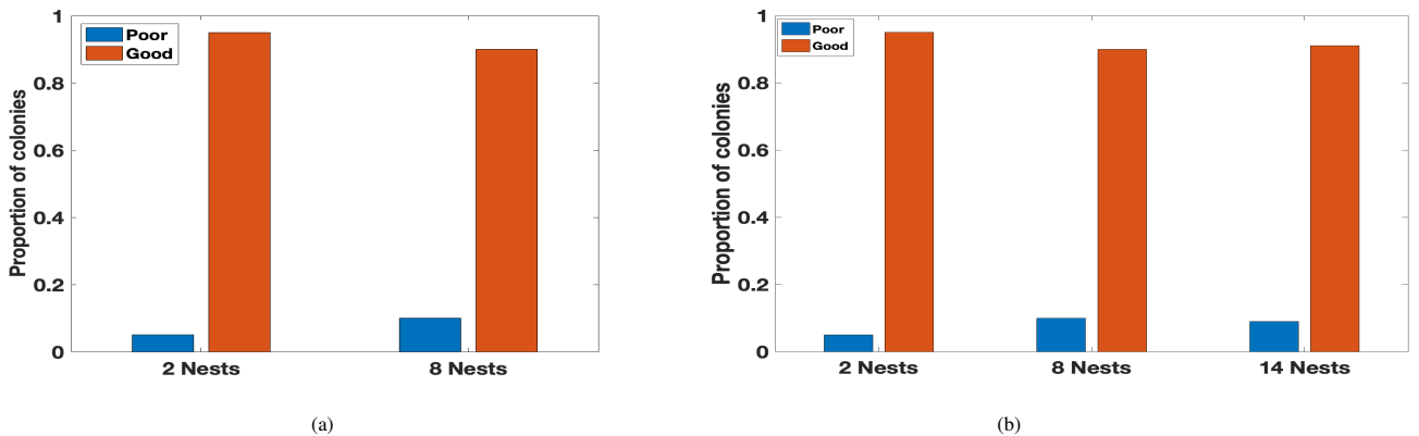
Figure A.3: The proportions of colonies that eventually moved into poor or good nests. (a): Empirical results in 2-nest and 8-nest settings [29]. (b): Simulation results from our model in 2-nest, 8-nest, and 14 nest settings.
