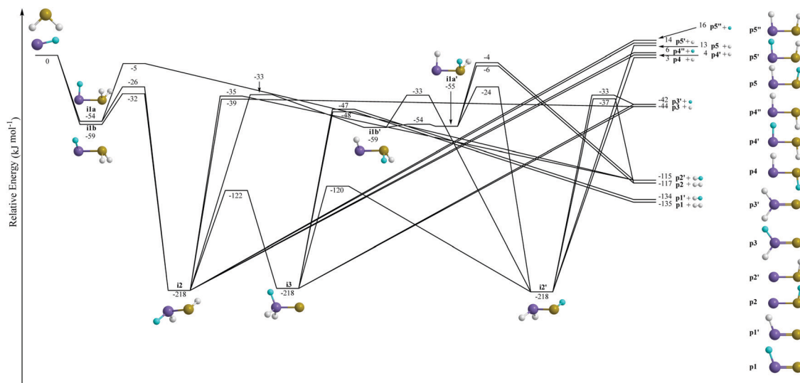
Fig. 12 Potential energy surface for the reaction of the D1-silyldyne radical (SiD; X^2\Pi ) with hydrogen sulfide ( H_2S ). Relative energies calculated at the CCSD(T)-F12/aug-cc-pV(T+d)Z//CCSD(T)/aug-cc-pV(T+d)Z+ZPE(M06-2X/cc-pV(T+d)Z) level of theory are shown in \text{kJ mol}^{-1} . The surface is simplified by removing barriers, intermediates, and most products above the collision energy of 15.6 \text{ kJ mol}^{-1} . Atoms are colored as follows: silicon (purple); sulfur (yellow); hydrogen (white); deuterium (light blue).
