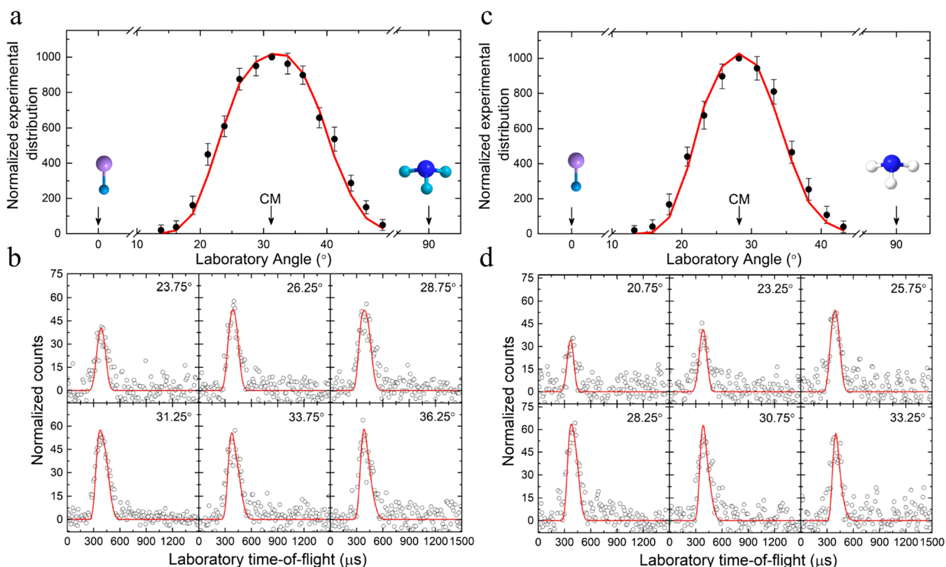
Figure 1. Laboratory angular distribution (a, c) and TOF spectra (b, d) for the reaction of the D1-silyldyne radical with D3-ammonia (data collected at m/z = 48 (a, b)) and with ammonia (data collected at m/z = 46 (c, d)). The solid circles define the experimental distribution; the open circles represent the experimental data; the red lines depict the best fits. Colors of the atoms: nitrogen, blue; silicon, purple; hydrogen, white; deuterium, light blue.
