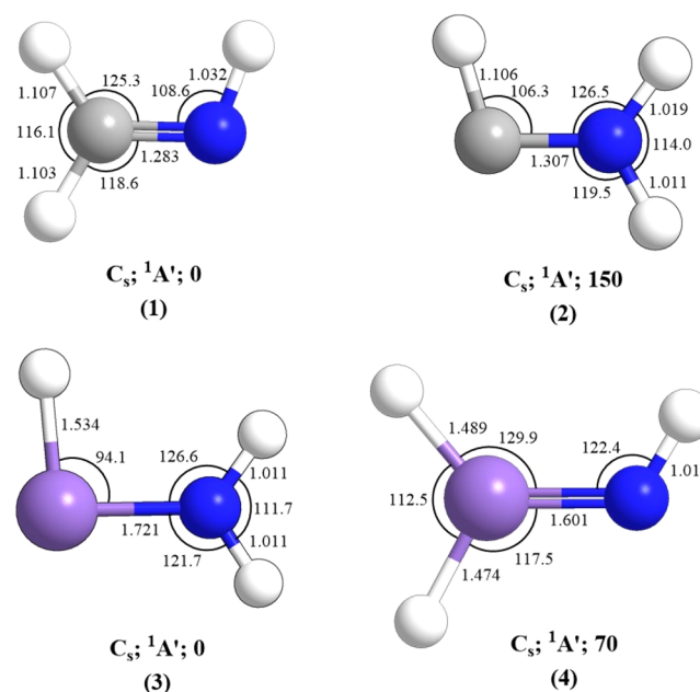
Figure 4. Geometries, point groups, electronic ground state wave functions, relative energies ( \text{kJ mol}^{-1} ), bond distances ( \text{\AA} ), and selected bond angles (degrees) of methanimine ( 1 , \text{H}_2\text{CNH} ) and aminomethylene ( 2 , \text{HCNH}_2 ) along with their isovalent species of aminosilylene ( 3 , \text{HSiNH}_2 ) and silanimine ( 4 , \text{H}_2\text{SiNH} ). Colors of the atoms: nitrogen, blue; silicon, purple; carbon, gray; hydrogen, white.
