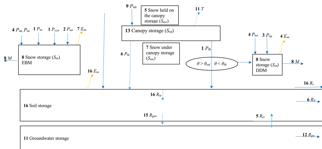
Figure 1. Scheme with number of models that compute vertical water balance in ISIMIP2b. Abbreviations are as follows. DDM: degree-day method; EBM: energy balance method; E_{sn} : sublimation; E_{so} : soil evaporation; M : snowmelt; P_{gr} : total precipitation falls directly to the ground; P_{int} : precipitation intercepted by canopy; P_{sn} : snowfall; P_{ra} : rainfall; P_{th} : throughfall; P_{tot} : total precipitation; P_{s,ca} : snowfall that is affected by the canopy interception and dripping; R_{cr} : capillary rise; R_{gw} : groundwater runoff; R_{gwr} : groundwater recharge; R_{if} : interflow; R_{in} : infiltration; R_s : surface runoff; T : transpiration; \theta : air temperature; \theta_{snf} : snow freeze temperature; \theta_M : melting temperature. Bold font indicates the number of models that compute water flows and water storage compartments in ISIMIP2b. Blue arrows show water flow, and orange arrows show evaporation.
