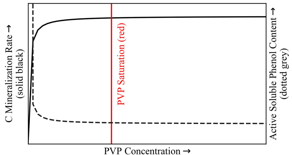
Fig 1. Hypothesized relationship between polyvinylpyrrolidone (PVP) concentration vs. C mineralization. C mineralization rate (measured by CO 2 and CH 4 production) corresponds to the primary y axis (solid black line). Assumed active soluble phenol content corresponds to the secondary y axis (dotted grey line). Addition of PVP was hypothesized to positively impact CO 2 and CH 4 production rates by inactivating soluble phenolics which would otherwise inhibit C decomposition. This relationship was expected to follow a Michaelis-Menten saturation curve. After reaching a point of PVP saturation (red line), further increases in PVP concentration were expected to yield no significant changes in C mineralization rates.
