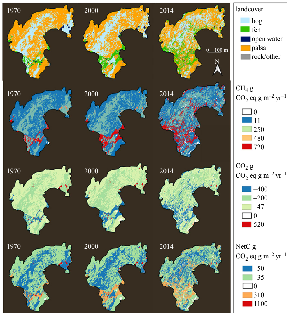
Figure 5. Time series of landcover, \text{CH}_4 , \text{CO}_2 and net radiative forcing represented as \text{g CO}_2\text{-equiv m}^{-2} \text{yr}^{-1} at Stordalen Mire, a permafrost peatland in northern Sweden for 1970, 2000 and 2014. See black outline in figure 1 for location. (Online version in colour.)
