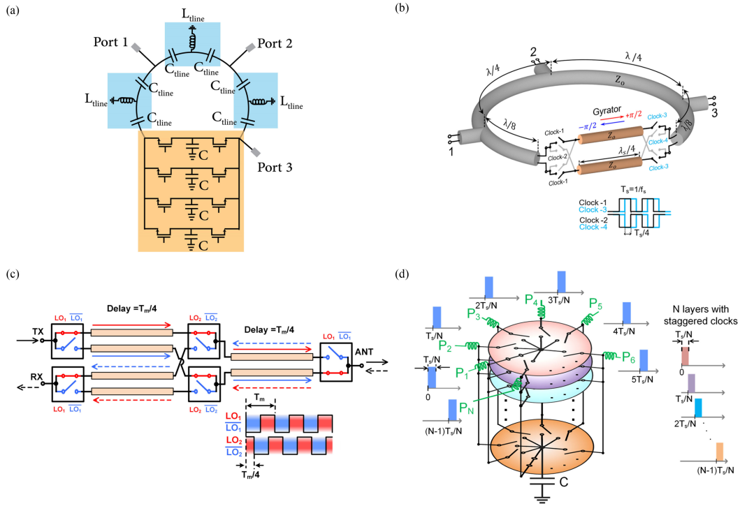
FIGURE 3. (a) CMOS circulator based on an N-path filter gyration employing commutation across a bank of capacitors [64]. (b) CMOS circulator based on switched transmission line gyration employing staggered commutation across delay lines [66]. (c) An ultra-wideband circulator based on sequentially-switched delay lines [67]. (d) CMOS based N-Way circulator realized using N-port switched capacitor layers [68].
