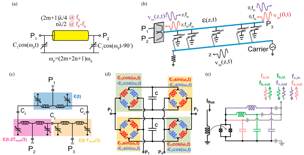
FIGURE 2. (a) Parametric non-reciprocal device based on temporal modulation of semiconductor-diode capacitances across a transmission-line delay [45]. (b) Non-reciprocal wave propagation accompanied by frequency conversion through traveling-wave permittivity modulation along a transmission line [46]. (c) Angular momentum biasing through permittivity modulation in coupled resonant rings [48]. (d) Superconducting, widely tunable microwave on-chip circulator based on DC SQUIDS [58]. (e) A superconducting, unidirectional frequency converter exploiting non-reciprocity in frequency space [59].
