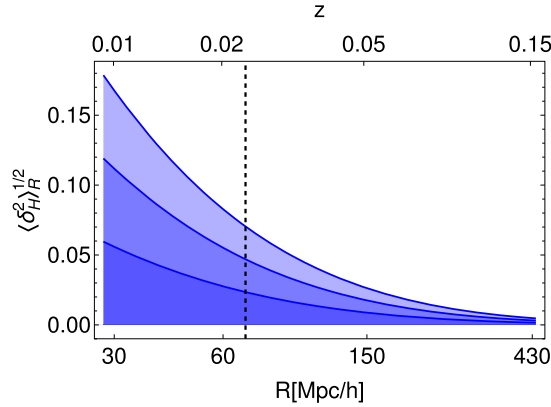
Fig. 3. 1, 2 and 3 times the standard deviation (\delta_H^2)^{1/2} as a function of redshift z and scale R(z) . The dashed line marks the redshift z = 0.023 . The Hubble constant is estimated by SH0ES in the redshift range 0.023 < z < 0.15 . Plot from Ref. (Camarena and Marra, 2018).
