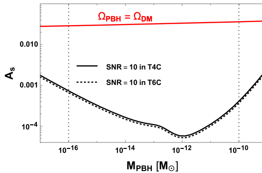
Fig. 17 Red curve: amplitude of the scalar power spectrum that gives the totality of the dark matter being PBH, as a function of the PBH mass. Black curves: minimal amplitude needed to have \text{SNR} = 10 at LISA for T4C (solid line) and T6C (dotted line). The dotted vertical lines denote approximately the mass range of interest: the lower bound originates from the \gamma background due to PBH evaporation, and the higher bound originates from lensing (Subaru HSC)
