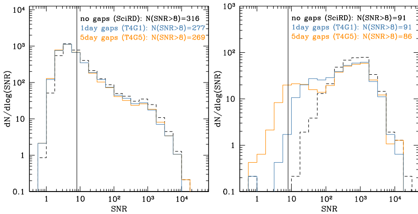
Fig. 1 SNR distribution for MBHBs in the popIII (left) and heavy seed (right) cases. In both scenarios we assume T_{\text{elapsed}} = 4 years. We compare observational scenarios with continuous data (SciRD) and data with gaps of different length and \mathcal{D} = 0.75 (T4G1, T4G5), as labeled in the figure. The legends show the number of sources observed with \text{SNR} > 8
