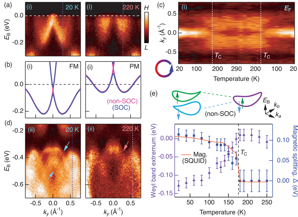
FIG. 2. Magnetic Weyl to Dirac loop collapse. (a) Cut (i) at 20 K and 220 K, with (b) corresponding ab initio calculation. Left: calculation in the ferromagnetic state through the Weyl loop, without SOC (magenta) and with SOC (blue). Right: calculation in the nonmagnetic state through the Dirac loop. (c) Momentum distribution curves (MDCs) of Cut (i) at the Fermi level for the full temperature cycle, 20 K \rightarrow 290 K \rightarrow 20 K. (d) Cut (ii), defined in Fig. 1(d), exhibiting clear splittings in deeper energy bands at 20 K (left), which collapse at 220 K (right). (e) Energy extremum of the Weyl loop band, extracted from the temperature dependence on Cut (i), obtained by Lorentzian fitting of energy distribution curves [EDCs, dotted lines in (a)]. Also, the magnetic exchange splitting as a function of temperature, obtained from Cut (ii) by Lorentzian fitting to EDCs [dotted lines in (d)] and compared with the magnetization M(T) . Cartoon: exchange gap collapse of two opposite-spin Weyl loop partners (blue and green) into a single Dirac loop (purple).
