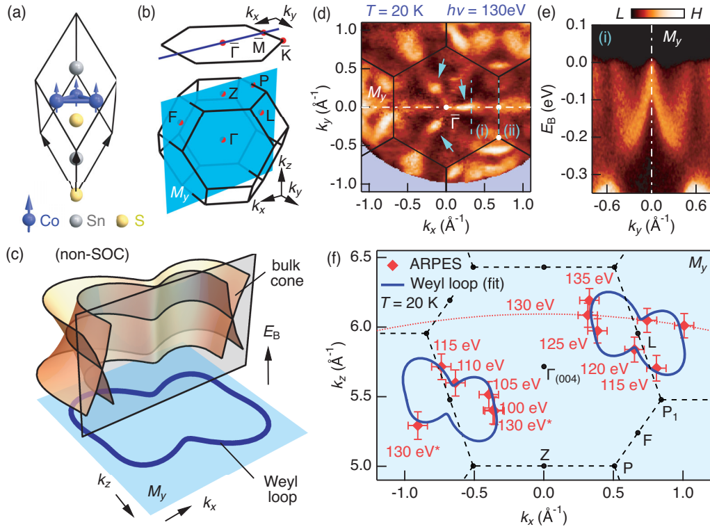
FIG. 1. Topological magnetic Weyl loop. (a) Primitive unit cell of ferromagnetic \text{Co}_3\text{Sn}_2\text{S}_2 , with mirror symmetry. (b) Bulk and (001) surface Brillouin zones with bulk mirror plane ( M_y , cyan) and several high-symmetry points (red). (c) In the absence of spin-orbit coupling (SOC), the combination of mirror symmetry and ferromagnetism generically gives rise to Weyl loops, which live in the mirror planes of the bulk Brillouin zone. A Weyl loop exhibits a ring of band crossings along a closed curve in momentum space (blue loop) with a linear cone dispersion on any energy-momentum slice through the loop. Under SOC, the Weyl loop typically gaps, possibly leaving behind Weyl points. (d) ARPES Fermi surface at T = 20 K and photon energy h\nu = 130 eV, exhibiting multiple dot features (cyan arrows) on the mirror planes ( \bar{\Gamma} - \bar{M} ). (e) Cone dispersion at the Fermi level on an energy-momentum spectrum through the dot feature (Cut (i)). (f) Collecting cone dispersions for a range of h\nu suggests a loop of band crossings (red diamonds) living in M_y and encircling the bulk L point (Figs. S4, S5). Different h\nu sample different out-of-plane k_z momenta; representative example shown for 130 eV (dotted red curve). The crossing points can be fit by a low-order polar coordinate Fourier decomposition around the L point (blue curve [53]), mapping out the trajectory of the Weyl loop.
