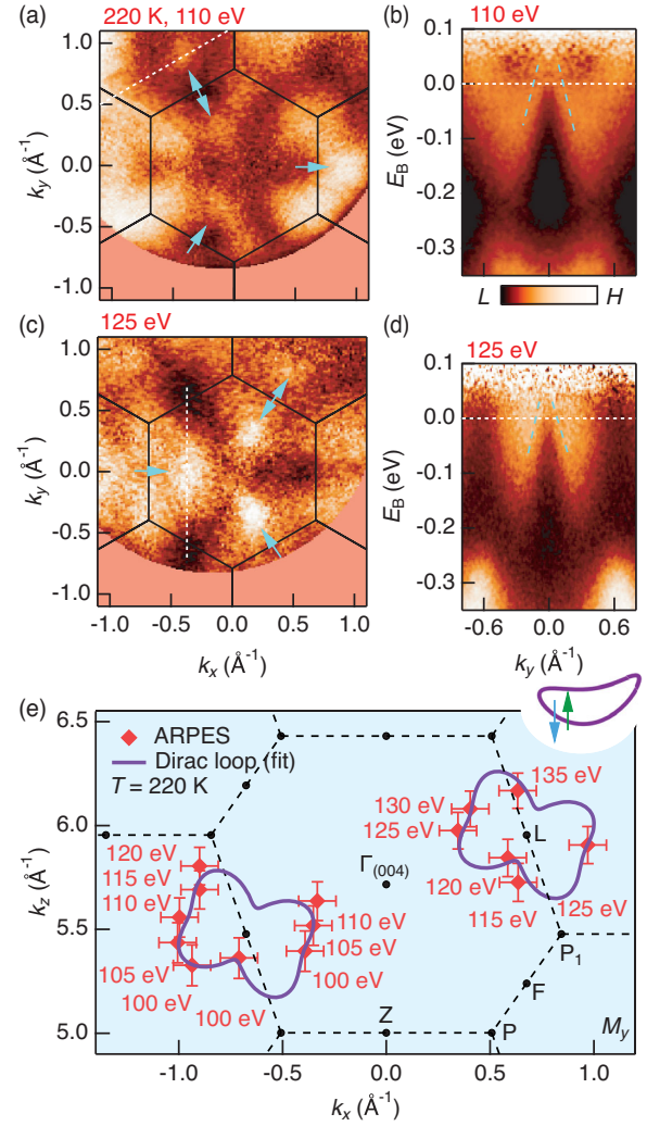
FIG. 3. Paramagnetic Dirac loop. (a) ARPES isoenergy contour slightly above E_F , at h\nu = 110 eV, acquired at 220 K, exhibiting pointlike features (cyan arrows) along \Gamma - M (corresponding to M_y and the symmetry-related mirror planes). (b) Energy-momentum cut through the pointlike feature, exhibiting conelike spectral weight [cut location: white line in (a)]. (c), (d) Analogous to (a), (b), at 125 eV. (e) Locations of cones observed for all h\nu (red diamonds, Fig. S7). Cones on symmetry-related mirror planes are plotted all together in a single momentum-space mirror plane M_y . Data points fit to a low-order polar coordinate Fourier decomposition around L (purple curves), mapping out the trajectory of the Dirac loop.
