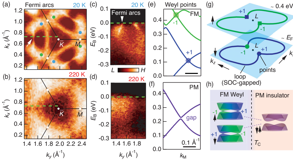
FIG. 4. Evidence for Fermi arc and Weyl point annihilation. (a) Fermi surface acquired at T = 20 K, h\nu = 130 eV, exhibiting candidate Fermi arc surface states (white arrow) near the Weyl point locations, as predicted by ab initio calculations (blue, green circle; Fig. S9). Data symmetrized for clarity. (b) Analogous Fermi surface at 220 K, with no signature of Fermi arcs. (c) Energy-momentum cut through the candidate Fermi arcs at 20 K [green dotted line, (a)]. (d) Analogous cut at 220 K. (e) Calculation in the ferromagnetic state, in the presence of SOC, slicing through a pair of exchange-split Weyl points of opposite chirality. (f) Analogous calculation, nonmagnetic state. The two partner Weyl points annihilate, opening a gap of 12 meV. (g) Schematic of the ferromagnetic Weyl loop (non-SOC) and Weyl point (SOC) configuration. (h) Schematic phase diagram: spin-orbit gapped ferromagnetic Weyl loops collapse to a paramagnetic Dirac loop across T_C . Concurrently, the exchange-split Weyl points annihilate.
