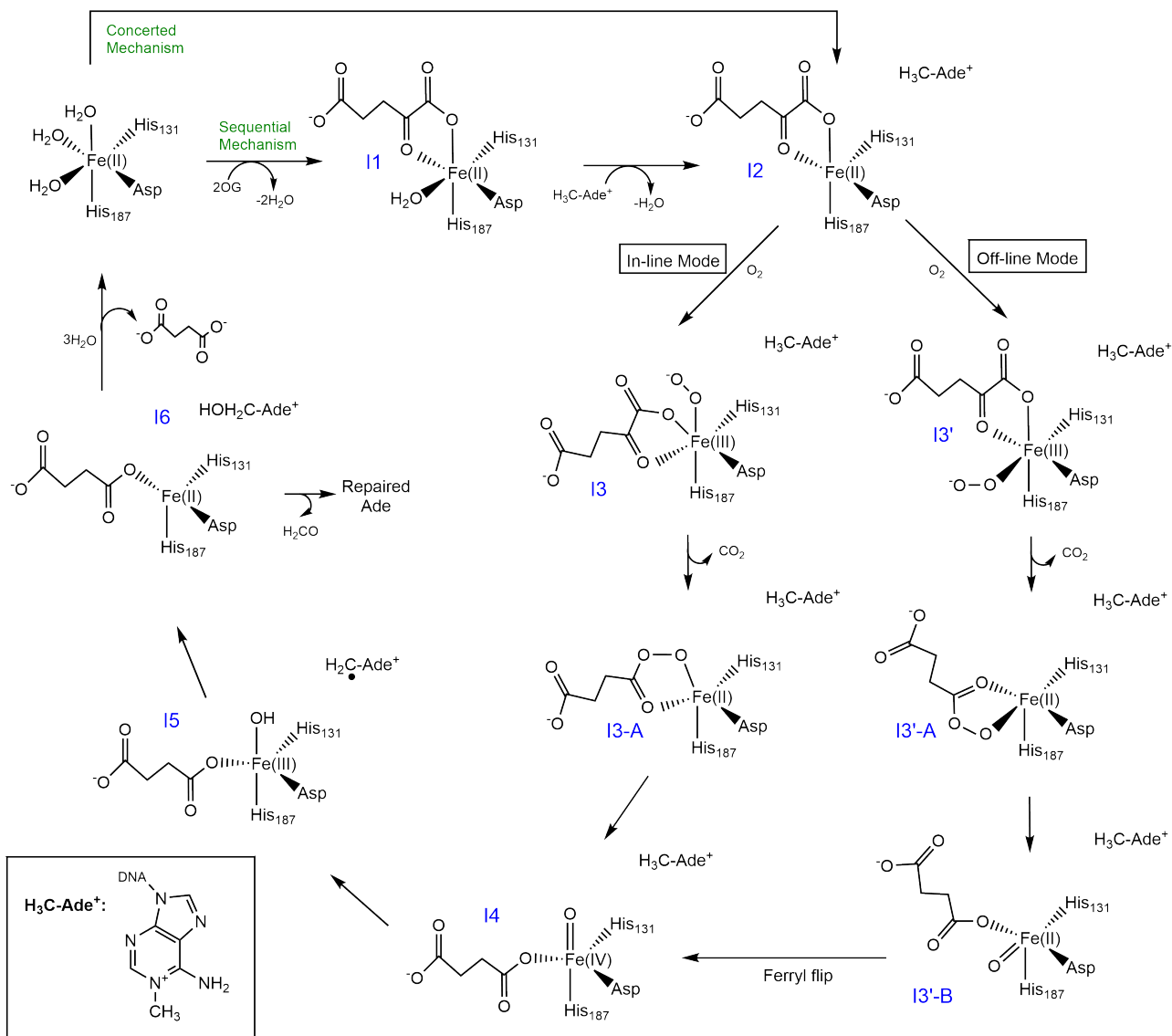
Scheme 1 The proposed AlkB catalyzed dealkylation mechanism of 1mA adapted from Waheed et al. 48
