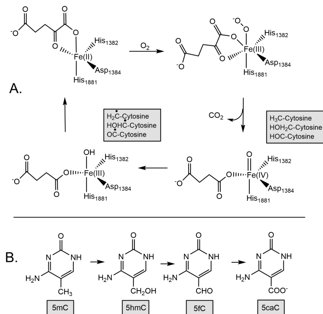
Scheme 3 (A) The demethylation reaction carried out by TET2 and (B) the sequence of methylated cytosine bases resulting from one round of oxidation.
