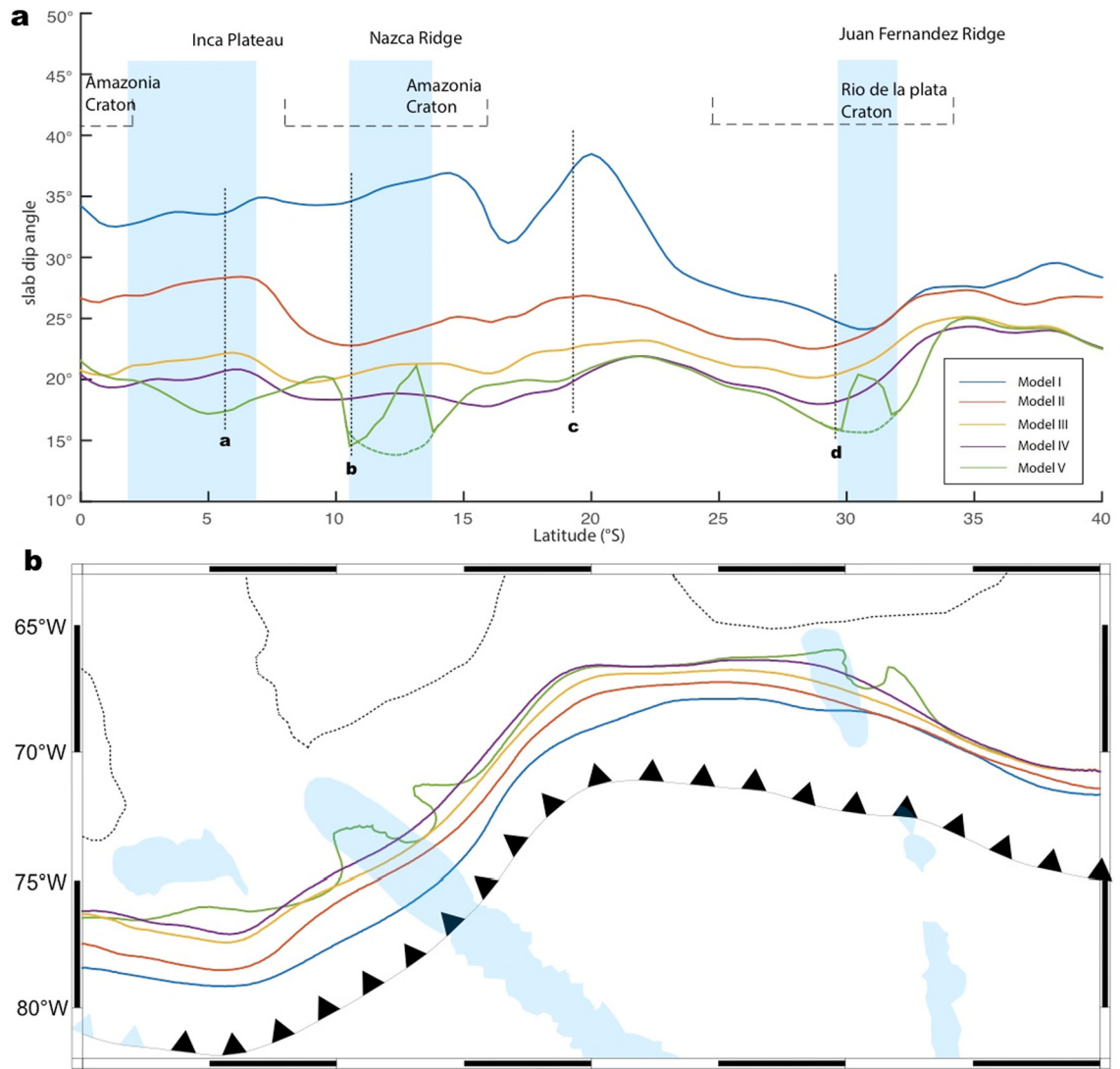
Fig. 5. (a) Present-day slab dip angle distribution along South American trench in models I, II, III, IV and V. The locations of subducting buoyancy features are marked with light blue, while the location of continental cratons are shown with dashed brackets. The dotted lines mark the location of the cross sections shown in Fig. 6. (b) Slab upper surface (300 °C cooler than the ambient mantle) at 200 km depth for the five models. Dashed lines outline the cratons, and light blue represents the buoyancy features. (For interpretation of the references to color in this figure legend, the reader is referred to the web version of this article.)
