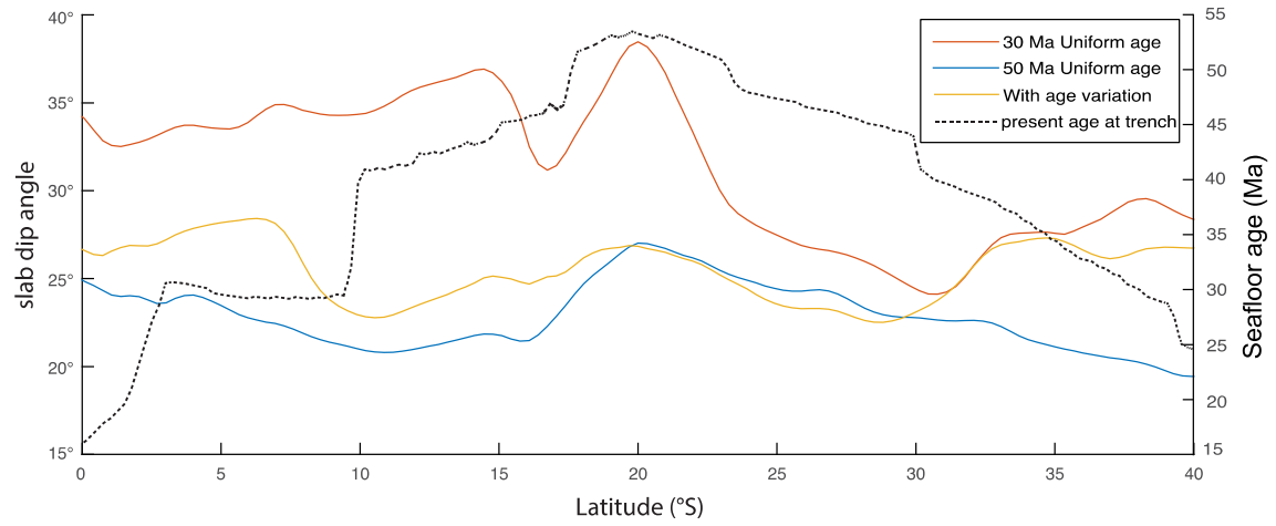
Fig. 4. Along-trench slab dip angle distribution (solid lines) from models I, II, and S and the present-day seafloor age distribution at trench (dashed line) in model II. Note the similar seafloor age distributions from 10 Ma to the present, the period relevant to the modern flat slab formation. Slab dip angle is measured according to the horizontal distance between the trench and the slab surface at 200 km depth along the east–west direction. Slab surface is defined as the upper interface between the slab and the ambient mantle, where the interface is the isotherm of 300 °C cooler than the ambient mantle.
