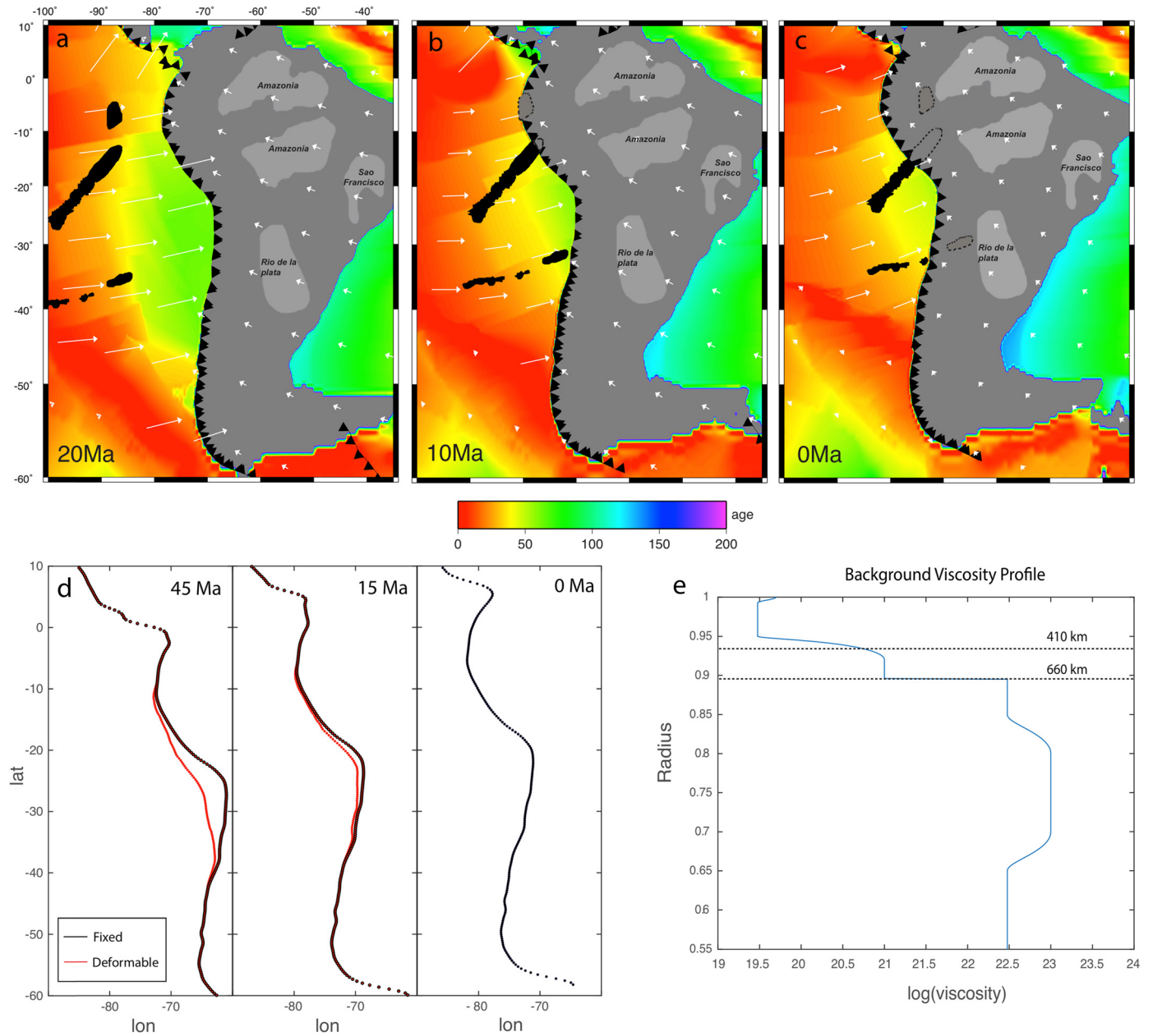
Fig. 2. Surface velocity boundary conditions and seafloor age distribution at (a) 20 Ma, (b) 10 Ma and (c) present. White arrows show the direction and magnitude of surface velocities. Background color represents the seafloor age. Black regions represent the oceanic plateau and aseismic ridges with dashed contours indicating the already-subducted parts. The South American continent is shown with dark gray with cratons indicated by light gray. (d) Trench profiles at 45 Ma, 15 Ma and present. Red lines indicate the temporally deformable trench profiles (Arriagada et al., 2008), and black lines represent the present-day trench geometry. (e) Background 1D mantle viscosity structure. Key features include a low-viscosity asthenosphere and a viscosity maximum in the upper part of the lower mantle. (For interpretation of the references to color in this figure legend, the reader is referred to the web version of this article.)
