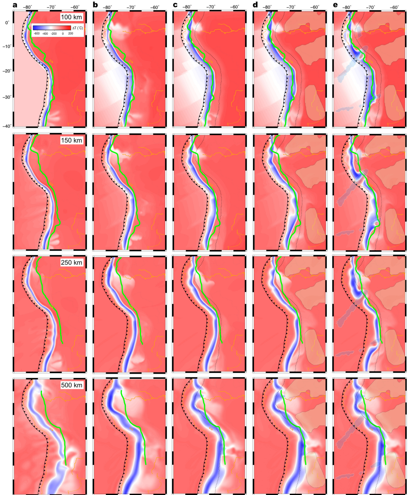
Fig. 3. Comparison of present-day slab geometry from five different subduction models. (a–e) Predicted slab geometry (blue color) from models I, II, III, IV and V (see main text), respectively. Different rows show different depths with the first row at 100 km, the second at 150 km, the third at 250 km, and the fourth at 500 km depth. Green lines represent the interpolated Benioff zones from slab 1.0 (Hayes et al., 2012). Present-day configuration of the cratons and buoyancy features are shown with brown and blue, respectively, where we assume no lateral distortion in the geometry of the buoyancy features after subduction. Dotted lines outline the overriding plate. Note the progressive flattening of the slab from model I to model V. (For interpretation of the references to color in this figure legend, the reader is referred to the web version of this article.)
