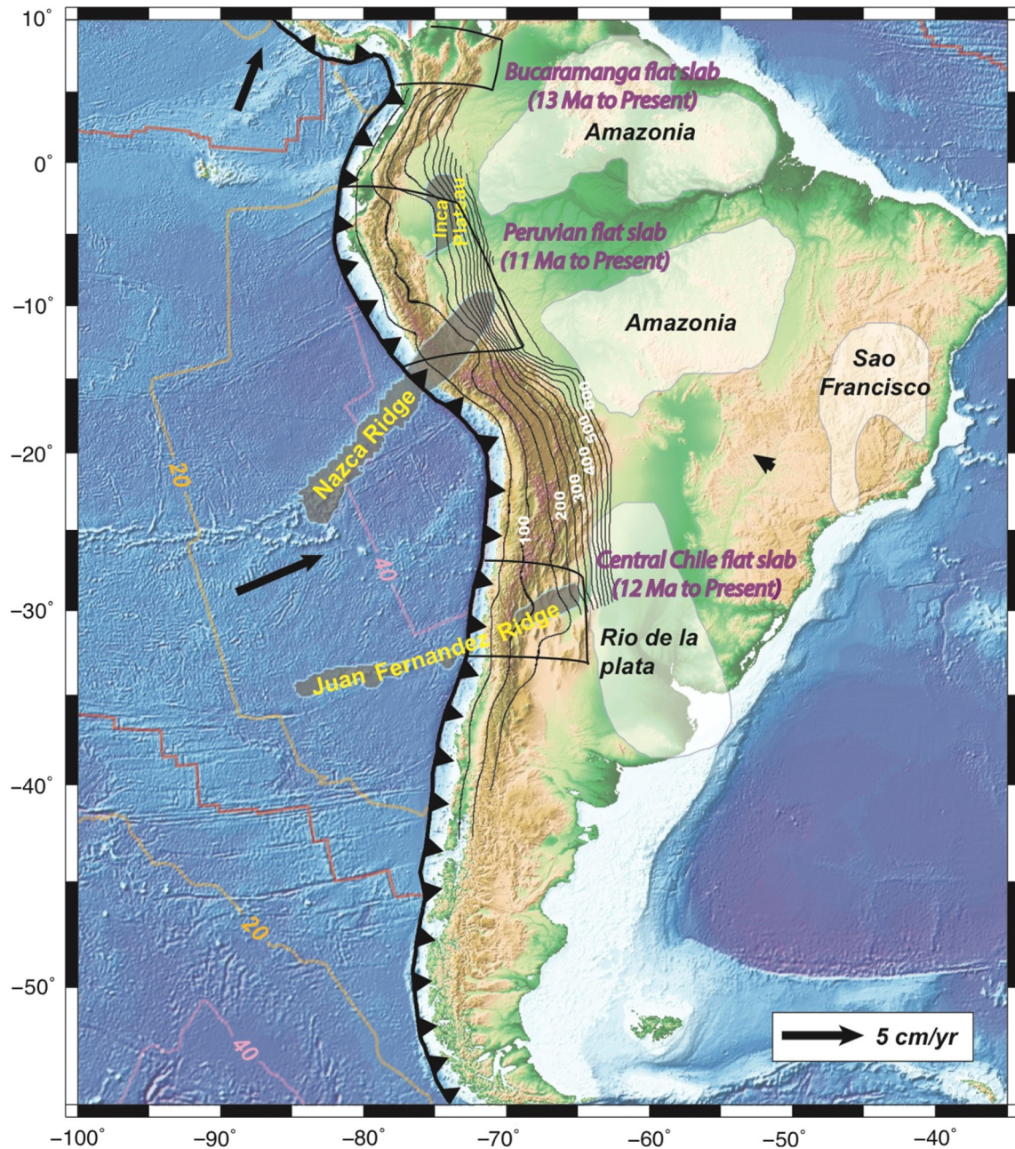
Fig. 1. Geological setting of South America with depth contours of slab 1.0 (Hayes et al., 2012) indicated by thin black lines, subducting oceanic plateaus translucent gray and continental cratons translucent white. The major flat slabs in South America are outlined with thick black lines. The locations of oceanic plateaus, cratons and flat slabs are modified from Gutscher et al. (2000), Loewy et al. (2004) and Ramos and Folguera (2009), respectively. The present-day plate motion is shown as black arrows. Tooth-shaped line represents the South American trench. Seafloor ages to the west of South America are shown with colorful lines with numbers indicating the age in Ma.
