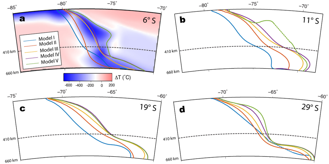
Fig. 6. Comparison of the slab upper surface of models I, II, III, IV and V at (a) 6°S, (b) 11°S, (c) 19°S and (d) 29°S, respectively, corresponding to the dashed lines in Fig. 5a. Notice the progressive flattening of the slabs across different models.
