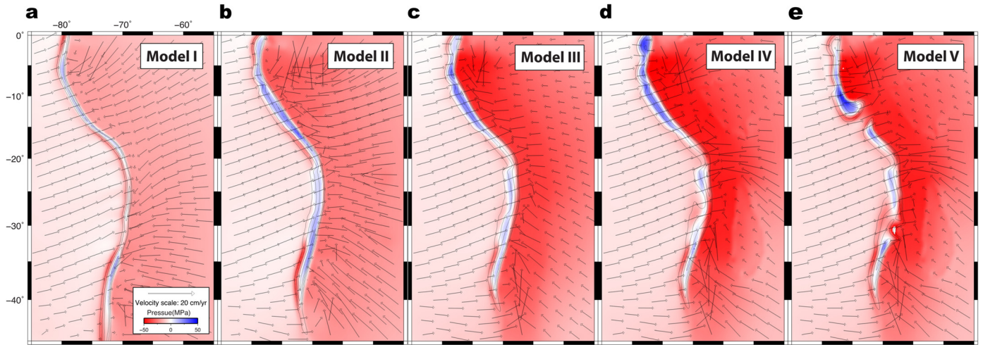
Fig. 7. Maps showing the dynamic pressure distribution at 140 km depth for models (a) I, (b) II, (c) III, (d) IV and (e) V. The mantle flow field is over-plotted as arrows. Thin black contours indicate slab isotherms with an increment of 100°C. The dynamic pressure in mantle wedge is progressively lowered from model I to model IV.
