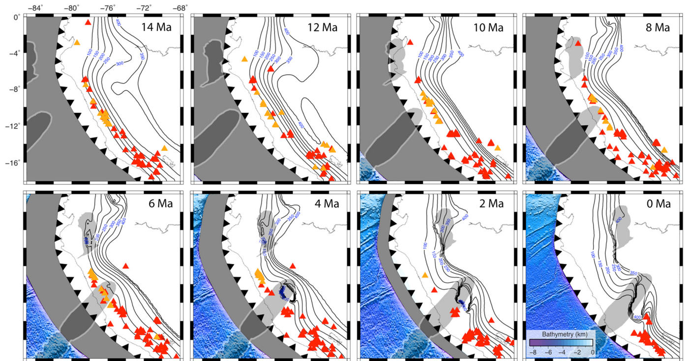
Fig. 9. The evolution of slab geometry beneath Peru from 14 Ma to present day. Black lines represent the slab upper surface (300 °C cooler than the ambient mantle) at different depths. Dark gray patterns show the reconstructed locations of the Inca Plateau and the Nazca Ridge. Light gray area represents now-subducted seafloors. Red triangles indicate the location of extrusive volcanism, while orange triangles represent that of intrusive volcanism. A slab hole forms since 6 Ma during the Nazca Ridge subduction. Note the delay between initial buoyancy feature subduction and flat slab formation. (For interpretation of the references to color in this figure legend, the reader is referred to the web version of this article.)
