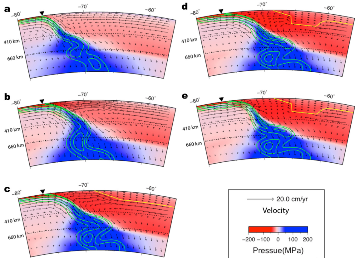
Fig. 8. Cross sections showing the dynamic pressure distribution at 15°S for model (a) I, (b) II, (c) III, (d) IV and (e) V. Arrows represent mantle velocities. Yellow thick lines outline the overriding plate. Solid green contours indicate slab isotherms with an increment of 100 °C. The dynamic pressure within the mantle wedge is progressively lowered from model I to model IV, indicating an increasing hydrodynamic suction. Notice that the mantle flow above the slab is mainly concentrated in the asthenosphere when a high-viscosity overriding plate is present. (For interpretation of the references to color in this figure legend, the reader is referred to the web version of this article.)
