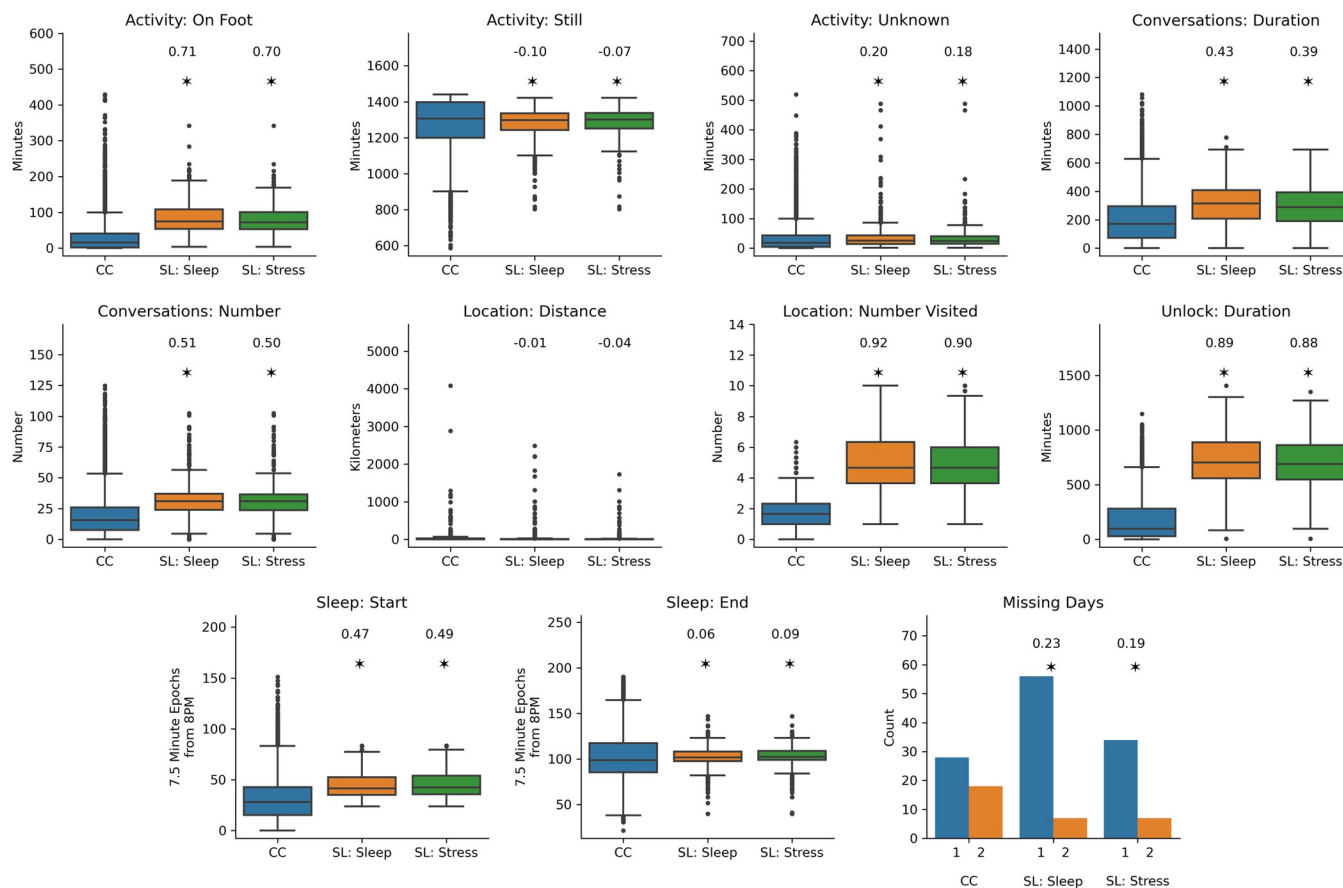
Fig 3. Example feature distribution differences across datasets. Assessing feature distributional differences across the CrossCheck (CC), StudentLife sleep EMA (SL: Sleep), and stress EMA (SL: Stress) validation data for an example 11 features across data types. Each subfigure shows a boxplot of the feature distribution within each specific dataset. The centerline of the boxplot is the median, the box edges the interquartile range (IQR), and the fences on the boxplot are values 1.5 x the IQR. The “Missing Days” distribution is a histogram, describing counts across participants. A “*” is listed above each of the StudentLife datasets if the distribution differed significantly (Mann-Whitney U test, two-sided, or Chi-square test of independence, \alpha = 0.05 ) from CrossCheck. The numbers above the “*” are the rank-biserial correlation (RBC) or Cramer’s V, which shows the magnitude of these differences. EMA: Ecological momentary assessment.
