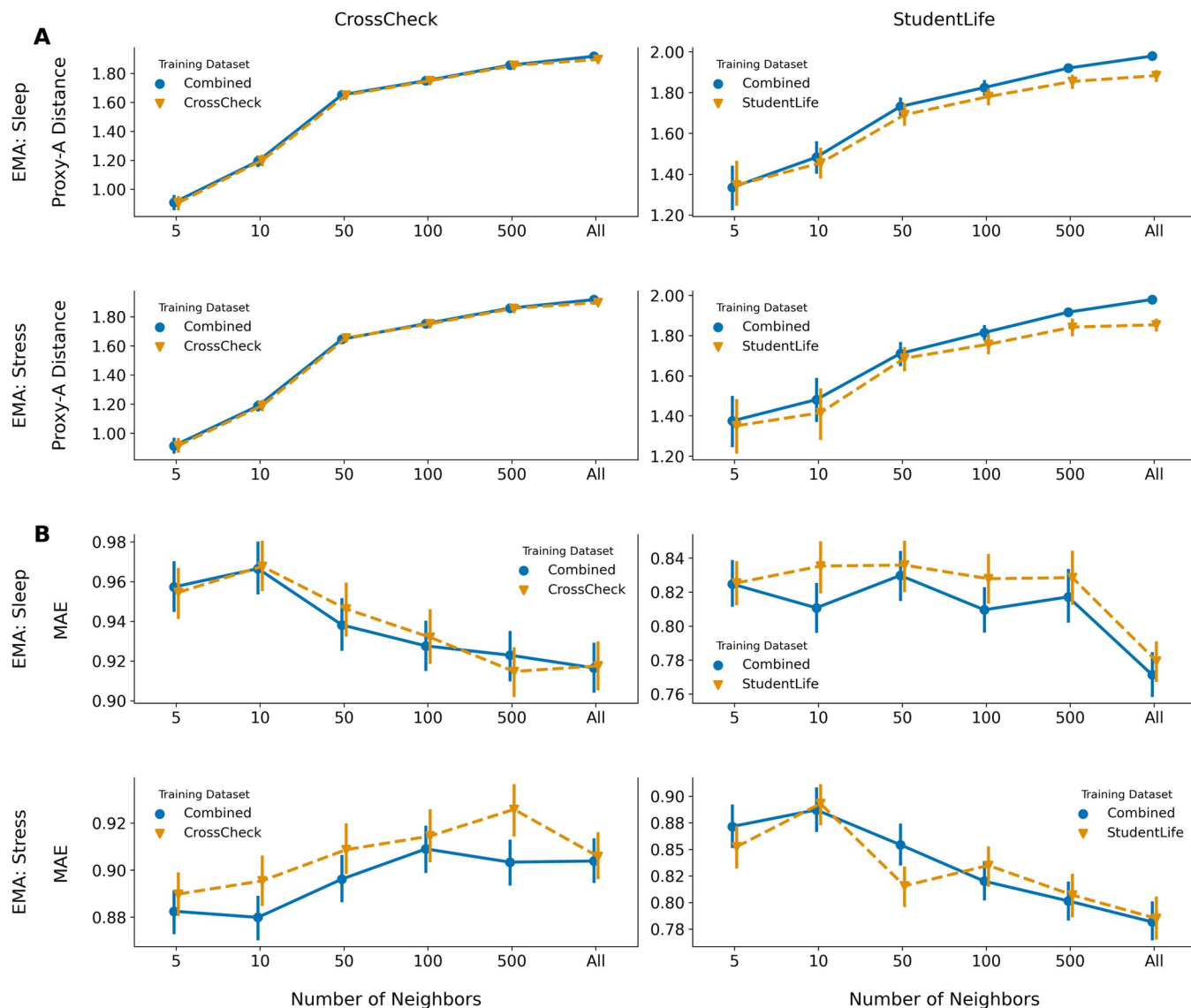
Fig 6. Personalization increases training and held-out data alignment, but is not guaranteed to improve prediction performance. (A) Effects of personalization by changing the number of neighbors (x-axis) used for model training on the feature distribution alignment between training and leave-one-subject-out cross-validation (LOSO-CV) participants (Proxy-A distance, y-axis). (B) Effects of changing the number of neighbors (x-axis) during model training on the model mean absolute error (MAE, y-axis). On all plots, each point is the mean Proxy-A distance (A) or MAE (B) across hyperparameters, and error bars are 95% confidence intervals around the mean. Each plot is split by the training data used (combined versus single-study), and plots are specific to the LOSO-CV result for a study (CrossCheck/StudentLife) and EMA (Sleep/Stress).
