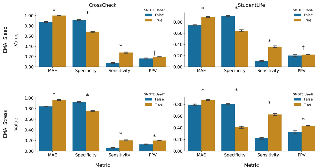
Fig 7. SMOTE increases sensitivity, positive predictive value, but reduces specificity and increases mean absolute error. SMOTE (see legends) oversampled under-represented ecological momentary assessment (EMA) values. The height of each bar is the mean value of the metric described on the x-axis across hyperparameters. Error bars are 95% confidence intervals around the mean. Plots are specific to the leave-one-subject-out cross-validation (LOSO-CV) result for a study (CrossCheck/StudentLife) and ecological momentary assessment (EMA) (Sleep/Stress). The specificity, sensitivity, and positive predictive value (PPV) were calculated by transforming regression results into a classification problem by labeling the two most severe symptom classes in each EMA with a “1” and other symptoms as “0”. Otherwise, the plots analyzed the regression mean absolute error (MAE). “*” indicates p < 0.05 , and “†” indicates p < 0.10 , for a Wilcoxon signed-rank test (one-sided) exploring differences using SMOTE/not using SMOTE across hyperparameter combinations.
