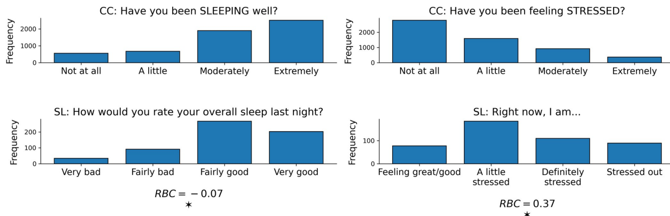
Fig 4. Outcome distribution differences across datasets. Sleep (left column) and stress (right column) ecological momentary assessment (EMA) validation distributions for CrossCheck (CC, top row) and StudentLife (SL, bottom row) data. The height of each bar represents the EMA response, where the specific response is listed on the x-axis under that bar. On the bottom, a “*” indicates whether there were significant (Mann-Whitney U test, two-sided, \alpha = 0.05 ) differences between CrossCheck and StudentLife EMA distributions, with rank-biserial correlation (RBC) values listing the magnitude of these differences.
