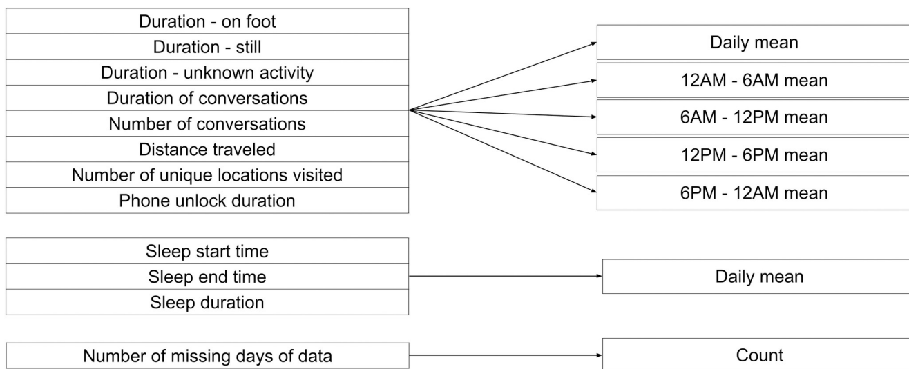
Fig 2. Summary of the 44 features used for prediction. Each data type on the left-hand side is summarized over a 3-day period for each epoch (e.g. 12AM - 6AM) using the aggregation technique (mean or count) described on the right-hand side. Aggregations were performed to align features with ecological momentary assessment (EMA) mental health symptom outcomes.
