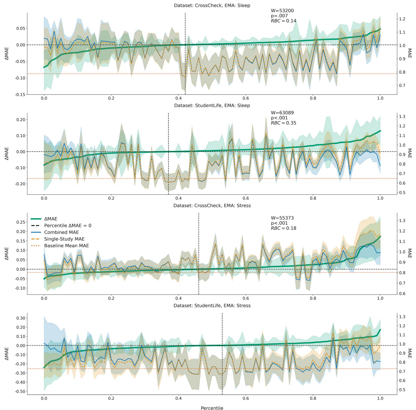
Fig 5. Sensitivity analysis reveals the combined versus single-study data is more likely to be predictive. The left y-axis describes the \Delta\text{MAE} = \text{MAE}_{\text{Single}} - \text{MAE}_{\text{Combined}} against the sorted distribution percentiles (x-axis). The thick green solid line represents the \Delta\text{MAE} percentiles, and the dashed black intersection lines show the percentile value (x-axis) where \Delta\text{MAE} = 0 . The right y-axis describes the actual MAE for the combined (blue solid line), and single-study (dashed orange line) data at each percentile. The baseline MAE, or error for a model predicting the average of the training data, is described by the dotted horizontal red line. Wilcoxon signed-rank test (one-sided) statistics (W), p-values, and rank-biserial correlations (RBCs) are included for models where across hyperparameters, using combined data significantly ( \alpha = 0.05 ) outperformed using single-study data (one-sided test). Shaded areas represent 95% confidence intervals around the mean. EMA: Ecological momentary assessment.
