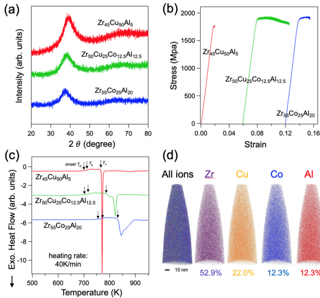
FIG. 2. Experimental (a) X-ray diffraction, (b) compression, (c) DSC, and (d) atom probe tomography data for (Zr_{45}Cu_{50}Al_5)_{1-x}(Zr_{55}Co_{25}Al_{20})_x ( x = 0, 0.5 , and 1).
