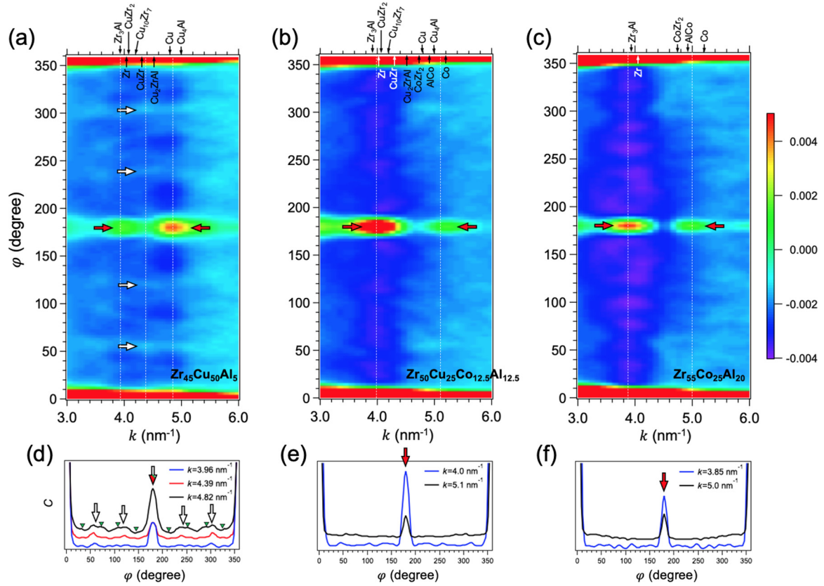
FIG. 3. Maps of averaged angular correlation, C(\varphi) , as a function of k , from (a) \text{Zr}_{45}\text{Cu}_{50}\text{Al}_5 ( x = 0 ), (b) \text{Zr}_{50}\text{Cu}_{25}\text{Co}_{12.5}\text{Al}_{12.5} ( x = 0.5 ), and (c) \text{Zr}_{55}\text{Co}_{25}\text{Al}_{20} ( x = 1 ). (d)–(f) The line profiles for different k values indicated with the white dashed lines on (a), (b), and (c), respectively. In (d), the profiles are shifted vertically for visual clarity.
