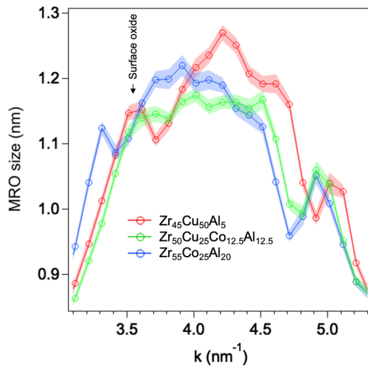
FIG. 4. Average MRO size vs. k from \text{Zr}_{45}\text{Cu}_{50}\text{Al}_5 ( x = 0 ), \text{Zr}_{50}\text{Cu}_{25}\text{Co}_{12.5}\text{Al}_{12.5} ( x = 0.5 ), and \text{Zr}_{55}\text{Co}_{25}\text{Al}_{20} ( x = 1 ). Color shadows indicate standard deviation of mean.
