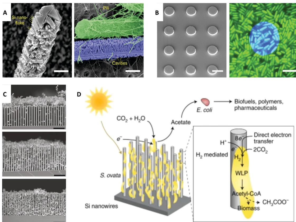
Fig. 5 Electrical-related interfaces with microbial systems. (A) Left: SEM image of mesostructured SiNWs with Si nanoflakes. Scale bar, 0.5 \mu\text{m} . Right: SEM image shows a strong interaction between the mesoscale cavities and the bacterial pili. Scale bar, 0.5 \mu\text{m} . (B) Left: SEM image of Si discs. Scale bar, 10 \mu\text{m} . Right: Confocal microscopy image shows Si disc (blue) on biofilms (green). Scale bar, 5 \mu\text{m} . (A) and (B) Reprinted with permission from ref. 130. Copyright 2020, AAAS. (C) SEM images of bacteria interfaced with nanowires. Top: Bacteria aggregation at pH 7.2. Middle: Semi-close packing at pH 6.7. Bottom: Fully packed hybrid structure at pH 6.4. Scale bar, 10 \mu\text{m} . Reprinted with permission from ref. 131. Copyright 2020, Elsevier. (D) Schematic representation of the functionality of photosynthetic S. ovata interfaced with nanowires. Biohybrid system converts CO 2 to acetate which can be turned into valuable chemicals with E. coli . Reprinted with permission from ref. 133. Copyright 2020, Springer Nature.
