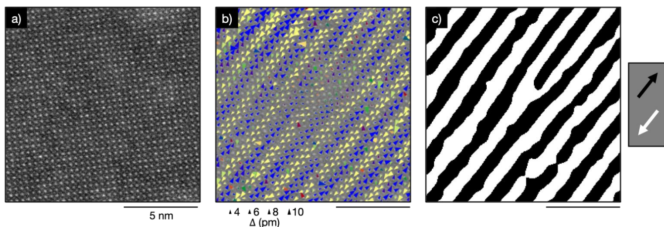
Figure 1. Measurement of a topological defect in a periodic lattice distortion (PLD) at \sim 115 K. a) Atomic resolution HAADF-STEM image shows a lattice free of crystalline defects. b) Map of picometer scale displacements of each atomic column in the low temperature phase reveal a topological defect in the PLD stripes. c) The defect and alternating directions of the stripes are highlighted by smoothing and thresholding the displacements from (b).
