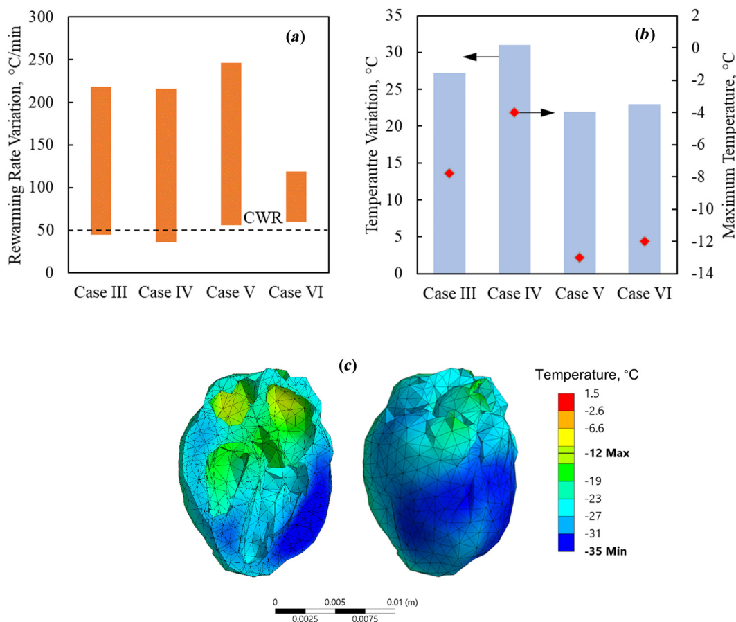
Fig. 5 Thermal results for the rat heart muscle contained in a cryobag for Cases III-VI: (a) rewarming rates range when the heart muscle temperature is between the glass transition temperature and the end of nanowarming, (b) temperature variation at the end of nanowarming when the lowest temperature in the heart surpasses -35^{\circ}\text{C} (bars), and the maximum temperature at the instant (red diamonds), and (c) temperature distribution superimposed on the heart model at the end of nanowarming for Case VI
