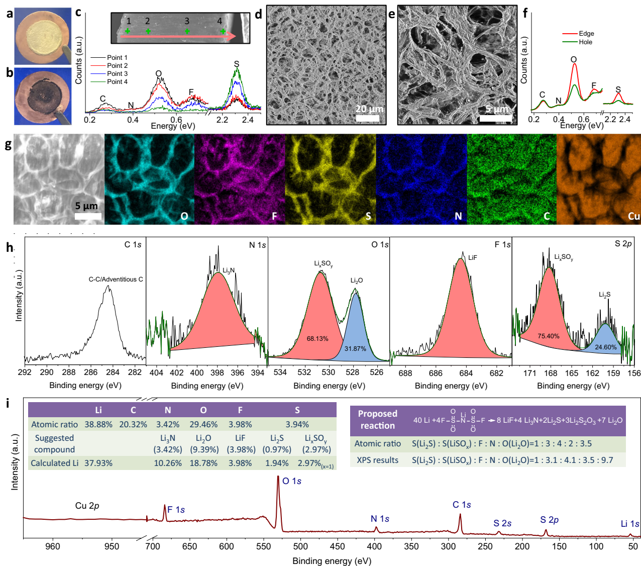
Fig. 4 Morphology and composition of the solid electrolyte interphase (SEI) formed on Li. Digital photos of a deposited lithium ( 20 \text{ mAh cm}^{-2} ) on Cu, and b material that remains after stripping lithium from Cu. c EDX spectra taken from the cross-section of deposited lithium from outer to inner edge (Marked points in the inset SEM image). d , e SEM image of the porous SEI left on Cu foil after stripping away the deposited Li. f Corresponding EDX spectra of SEI either on the edge or in the center of the pores of the residual porous material. g SEM-EDX O, F, S, C, N, Cu element mapping of SEI. h High-resolution XPS analysis of C 1s, N 1s, O 1s, F 1s, S 2p. i Atomic ratio analysis from XPS survey spectra with inserted supposed compositions and SEI formations process.
