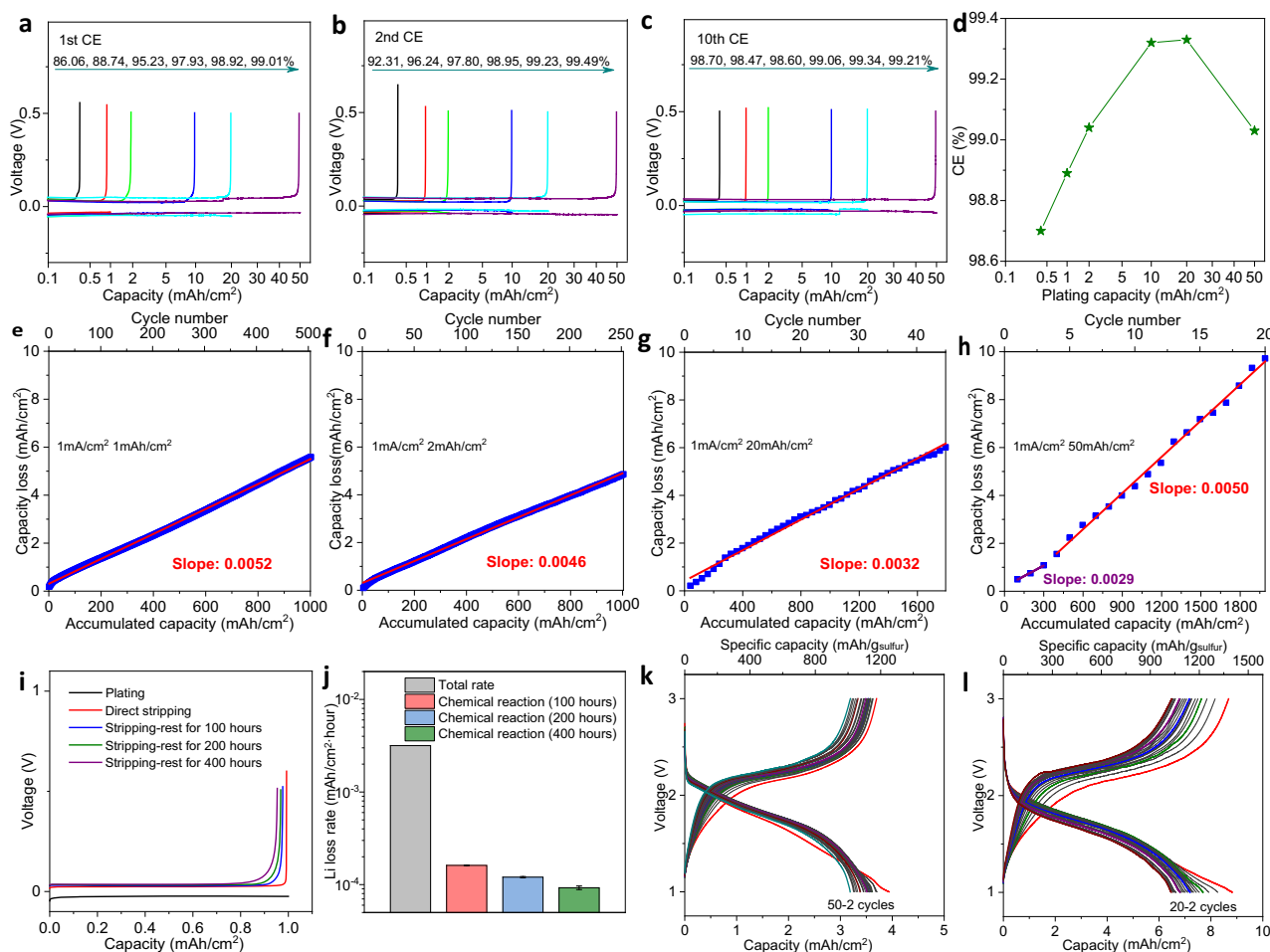
Fig. 3 Electrochemical reversibility of lithium as a function of Li plating capacity. a–c Galvanostatic lithium stripping/plating profiles for Li||Cu electrochemical cells. a First cycle, b Second cycle, c 10th cycle. The Li deposit capacities in a–c from low to high are 0.4 \text{ mAh cm}^{-2} , 1 \text{ mAh cm}^{-2} , 2 \text{ mAh cm}^{-2} , 10 \text{ mAh cm}^{-2} , 20 \text{ mAh cm}^{-2} , and 50 \text{ mAh cm}^{-2} , respectively. d Comparison of average CEs as a function of Li deposit capacity. e–h Rate of lithium consumption at various plating capacities. e 1 \text{ mAh cm}^{-2} , f 2 \text{ mAh cm}^{-2} , g 20 \text{ mAh cm}^{-2} , and h 50 \text{ mAh cm}^{-2} . The bottom X axis is the accumulated capacity for both stripping and plating. The top X axis reflects the number of lithium stripping/plating cycles. i Lithium plating/stripping profiles with or without resting after the plating process. j Comparison of total lithium consumption rate and consumption caused by spontaneous chemical reactions. The error bars (standard deviation) were calculated based on at least two sets of data. k–l Lithium-sulfur battery applications with high areal capacity lithium utilization per cycle (Current density: 0.5 \text{ mA cm}^{-2} ). Discharge/charge profiles of lithium-sulfur batteries coupled with high loading sulfur cathode and thin lithium metal anode ( k , 50 \mu\text{m} , l 100 \mu\text{m} ). All results from a to j were obtained at a fixed current density of 1 \text{ mA cm}^{-2} for both lithium stripping/plating processes. The electrolyte used is 2 \text{ M LiFSI} in DOL with 0.5 \text{ M LiNO}_3 .
