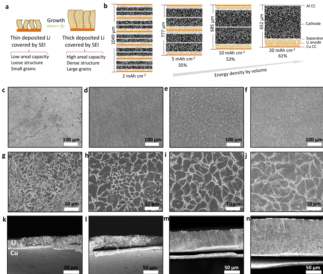
Fig. 1 Morphological transition at Li anode at high deposition capacity. a Proposed growth mechanism for lithium deposition at electrodes with areal capacity ranging from low to very high. SEI stands for solid electrolyte interphase. b Schematic illustrating impact of anode areal capacity on the overall energy density of Li metal full-cell batteries. A high-capacity cathode coupled with dense lithium deposition achieved at 20 \text{ mAh cm}^{-2} exhibits a 61% increase in volumetric energy density (See details in Methods). CC stands for the current collector. c–n Morphology evolution of deposited lithium metal from low to high areal capacity. c, g and k , 2 \text{ mAh cm}^{-2} ; d, h and i , 5 \text{ mAh cm}^{-2} ; e, i and m , 10 \text{ mAh cm}^{-2} ; f, j and n , 20 \text{ mAh cm}^{-2} . c–j top view; k–n cross-section view.
