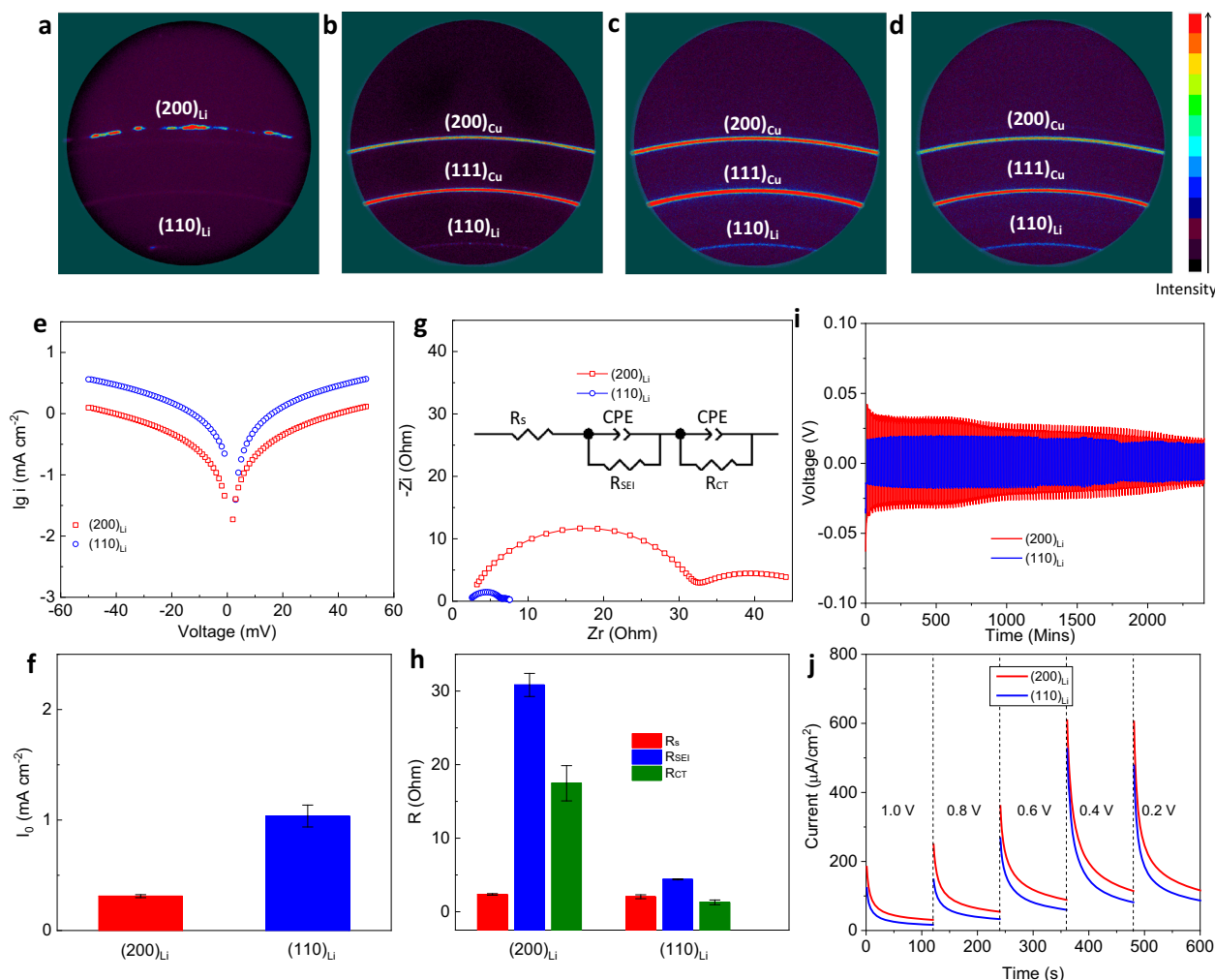
Fig. 2 Crystallography, morphology, and kinetics of deposited lithium metal at low, moderate, and high areal capacities. a–d 2D General area XRD analysis. a pristine lithium foil with (200) preferred crystal face orientation. b–d deposited lithium on Cu substrate with an areal capacity of 5 mAh cm −2 , c 10 mAh cm −2 , and d 20 mAh cm −2 , showing (110) preferred crystal facet orientation. e–j kinetic studies of (200) Li and (110) Li electrodes. e Tafel plots and f , corresponding exchanging current density. The error bars (standard deviation) were calculated based on at least two sets of data. g , EIS and h , bulk resistance ( R_s ), charge transfer resistance ( R_{CT} ), and SEI resistance ( R_{SEI} ) calculated by symmetrical Li||Li electrochemical cells. The error bars (standard deviation) were calculated based on at least two sets of data. i Lithium stripping/plating profiles of symmetrical Li||Li electrochemical cells. The current density used for lithium stripping/plating is 1 mA cm −2 . j Chronoamperometry measurements in Li||Cu electrochemical cells. The notation (110) Li is used here to denote deposited Li with a plating capacity of 20 mAh cm −2 . The notation (200) Li is used to denote Li foil obtained by electrochemically stripping 0.5 mAh cm −2 Li at a current density of 0.5 mA cm 2 , conditions where the Li foil can react with the electrolyte.
