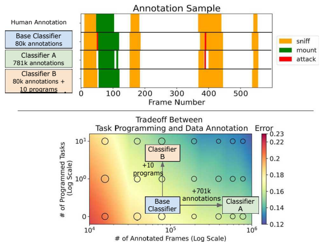
Figure 1. Overview of our approach. Part 1: A typical behavior study starts with extraction of tracking data from videos. We show 7 keypoints for each mouse, and draw the trajectory of the nose keypoint. Part 2: Domain experts can either do data annotation (Classifier A) or task programming (Classifier B) to reduce classifier error. The middle panel shows annotated frames at 30Hz. Colors in the bottom plot represent interpolated performance based on classifier error at the circular markers (full results in Section 4.3). The size of the marker represents the error variance.
