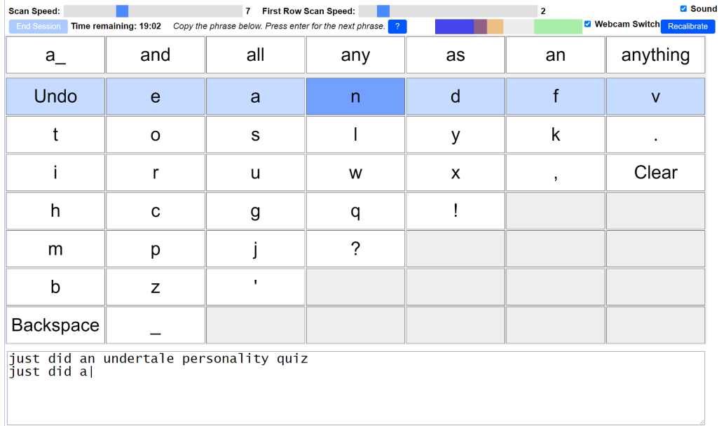
Figure 2: Our row-column scanning keyboard interface. The user is being prompted to write “just did an undertale personality quiz” and has written “just did a” so far. The interface progressively highlights rows until the user clicks their switch, and then progressively highlights columns within the selected row until the user clicks once more. Users can also select word completions that are displayed at the top.
