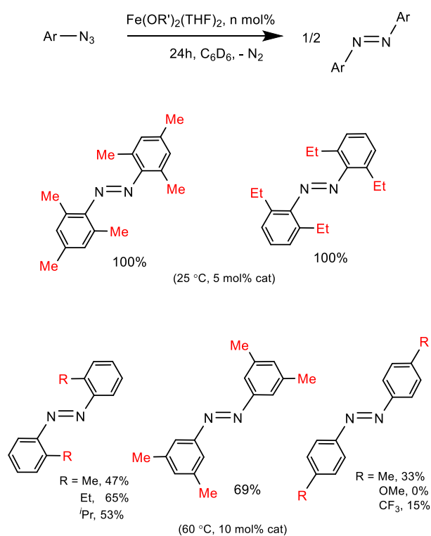
Fig. 14 Catalytic reactivity of \text{Fe}(\text{OR}')_2(\text{THF})_2 in nitrene homocoupling.
