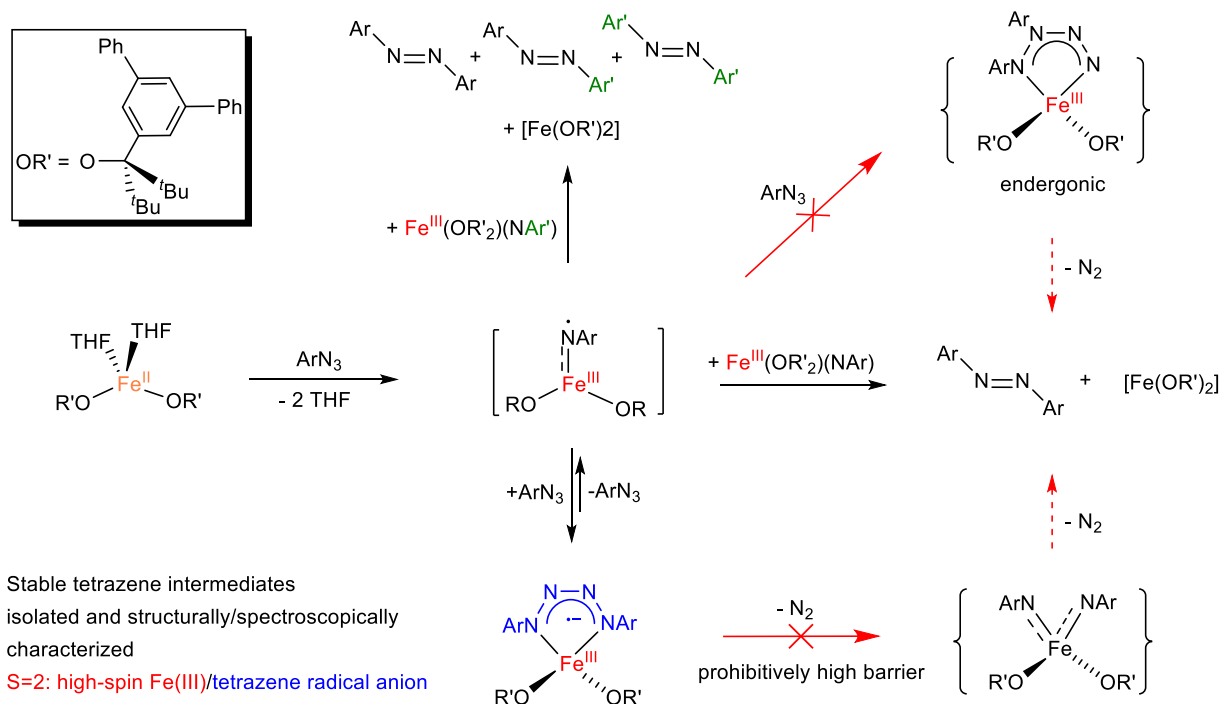
Fig. 15 Mechanistic studies on the reactivity of \text{Fe(OR')}_2(\text{THF})_2 with aryl azides.
