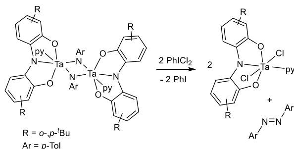
Fig. 5 Selected examples of nitrene homocoupling.
