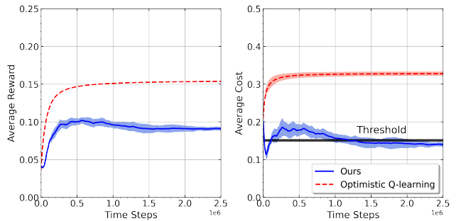
Figure 2: Average reward and cost of our algorithm during training, and the shaded region represents the standard deviations.
