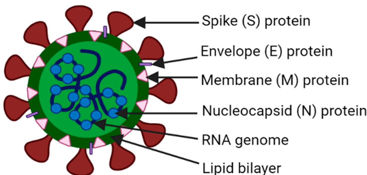
Figure 2. A typical virion structure of a coronavirus (created with BioRender.com. Accessed on 28 July 2021).
