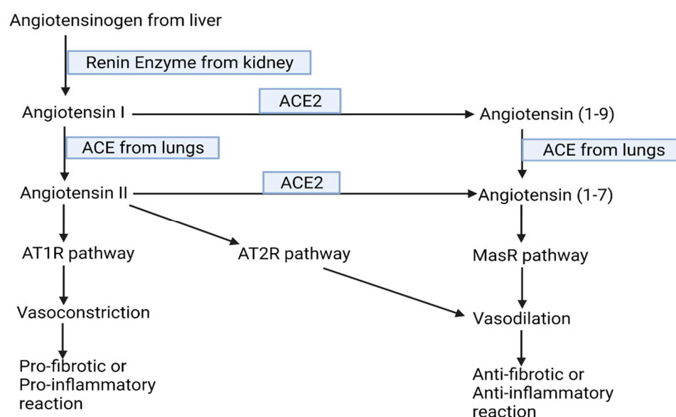
Figure 1. Flowchart of RAS. ACE, Angiotensin converting enzyme; AT1R, Angiotensin type 1 receptor; AT2R, type 2 receptor; MasR, Mas receptor. The boxes wrap the relevant enzymes catalyzing the reaction (created with BioRender.com. Accessed on 09 September 2021).
