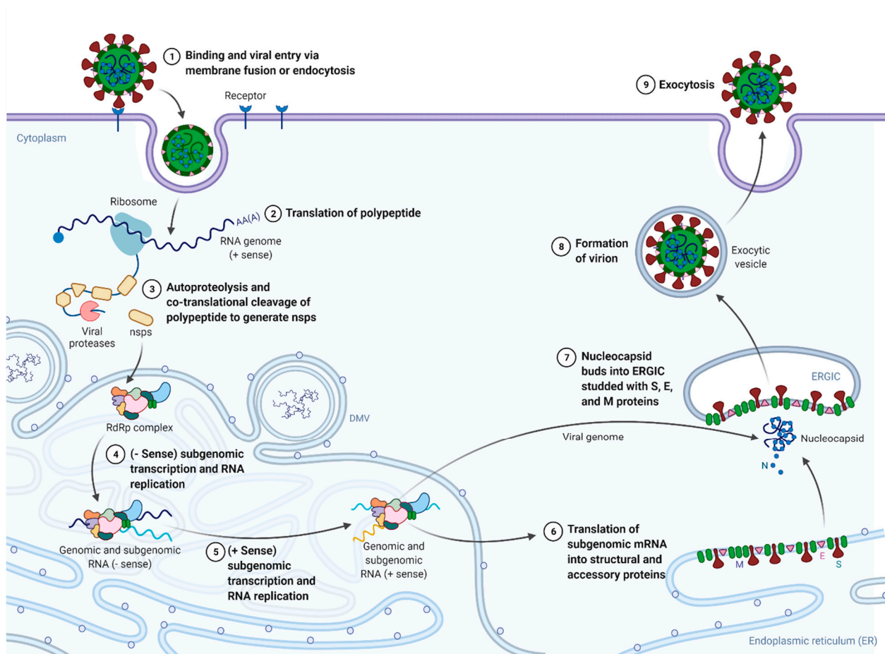
Figure 4. Major events in the life cycle of coronaviruses. Nsps, non-structural proteins; DMV, double membrane vesicles; ERGIC, endoplasmic reticulum-golgi intermediate compartment (created with BioRender.com. Accessed on 28 July 2021).
