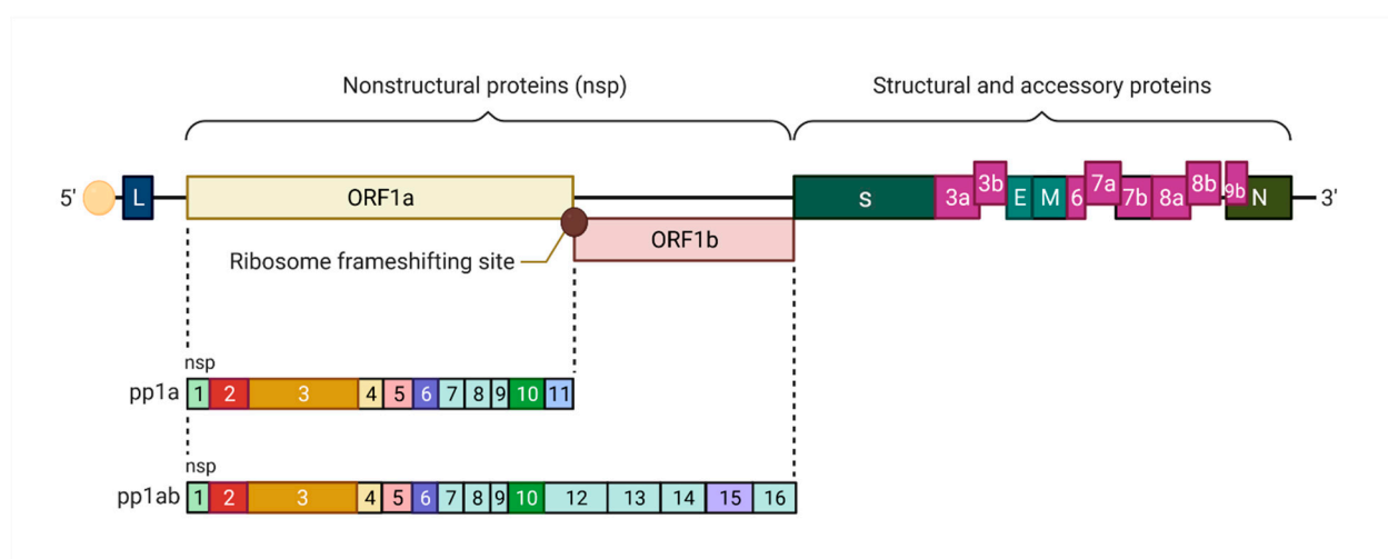
Figure 3. Genomic organization of SARS-CoV, where one third of the right part of the genome encodes nine accessory proteins (3a, 3b, 6, 7a, 7b, 8a, 8b and 9b). These are interspersed between genes encoding structural proteins (S, E, M, N). UTRs are flanking the RNA at both 5′ and 3′ ends. Capping represented by solid yellow and leader sequence indicated by L are at 5′-end. ORF, Open reading frame; UTR, Untranslated region (created with BioRender.com. Accessed on 07/28/2021).
