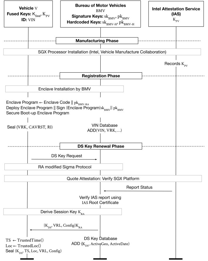
Fig. 1: Sequence diagram of the three phases of DS key design. The notation \{D\}_{key} denotes encryption of the any data D with the symmetric key K .
