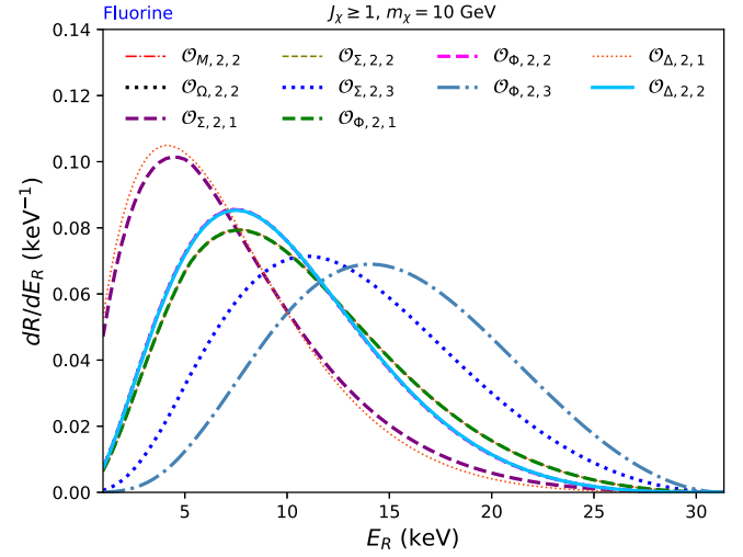
FIG. 3. Same as Fig. 1 but for a fluorine target.
