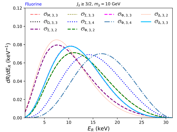
FIG. 4. Same as in Fig. 2 but for a fluorine target.
