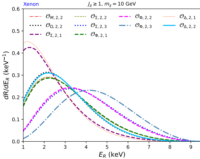
FIG. 1. Expected differential scattering rate (1.5) normalized to 1 event for a 10 GeV mass WIMP with a xenon target and for the 10 irreducible effective operators \mathcal{O}_{X,2,l} defined in Eqs. (3.22), assuming a WIMP of spin j_\chi \geq 1 .
