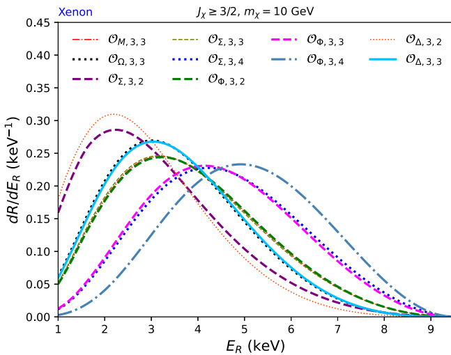
FIG. 2. Same as Fig. 1 but for the 10 irreducible effective operators \mathcal{O}_{X,3,l} and assuming a WIMP of spin j_\chi \geq 3/2 .
