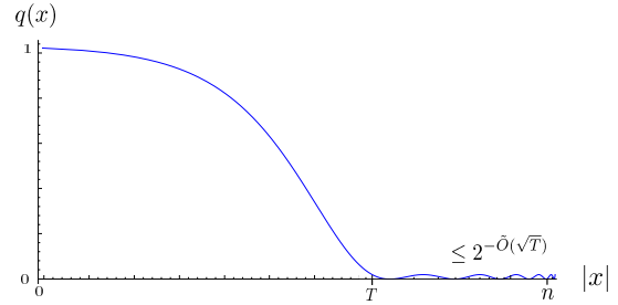
Figure 3: Caricature of the polynomial q(x)
