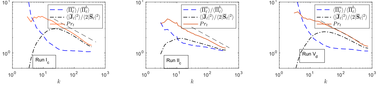
Figure 8. Plots showing the turbulent magnetic Prandtl number Pr_t and its two components \langle \bar{\Pi}_\ell^u \rangle / \langle \bar{\Pi}_\ell^b \rangle and \langle |\bar{\mathbf{J}}_\ell|^2 \rangle / \langle 2|\bar{\mathbf{S}}_\ell|^2 \rangle at the highest resolutions of Run I, II, and V (ABC forcing) in Table 1. A reference line with a slope of -1/3 (black dashed) is added. The plots show that \langle \bar{\Pi}_\ell^u \rangle / \langle \bar{\Pi}_\ell^b \rangle approaches a constant in the decoupled range. Note that with a strong external B-field (Run II), we expect \langle \bar{\Pi}_\ell^u \rangle / \langle \bar{\Pi}_\ell^b \rangle to plateau at sufficiently high Reynolds numbers (Bian & Aluie 2019).
