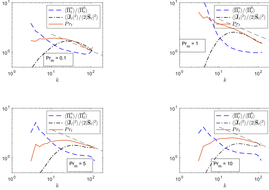
Figure 3. Plots showing Pr_t and its two components \langle \bar{\Pi}_\ell^u \rangle / \langle \bar{\Pi}_\ell^b \rangle and \langle |\bar{\mathbf{J}}_\ell|^2 \rangle / \langle 2|\bar{\mathbf{S}}_\ell|^2 \rangle using unity ( Pr_m = 1 ) and non-unity microscopic Prandtl numbers ( Pr_m = 0.1, 5, 10 ) on 512^3 grid. See parameters in Table 1. A reference line with a slope of -1/3 (black dashed line) is added.
