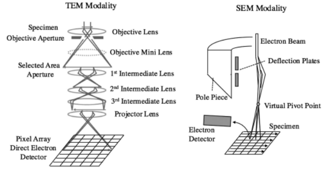
Fig. 2. Illustration of the transmission and scanning electron microscopy image acquisition process. We approximate both image acquisition processes by block-averaging a HR image as described in Section II-B. The scanning electron microscopy image shown is adapted from [26].
