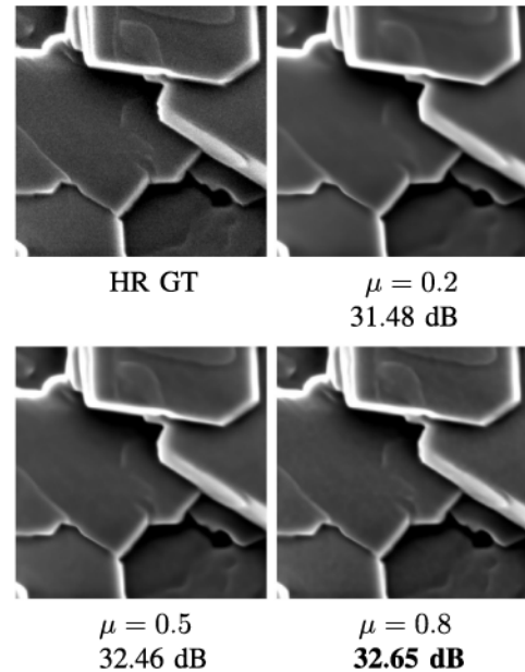
Fig. 6. Left : Plot of intensities along the blue segment for selected reconstructions from Fig. 5. DPSR produces the sharpest edge boundary, while PnP and MDF-RAP better approximate GT image on crystal edges. Right : Comparison of 4x super-resolution reconstructions of a simulated LR EM image of pentacene crystals at varying regularization levels. Note as \mu increases, more detail is present in the final reconstruction. However this can introduce textural artifacts from the forward model into the final reconstruction.
