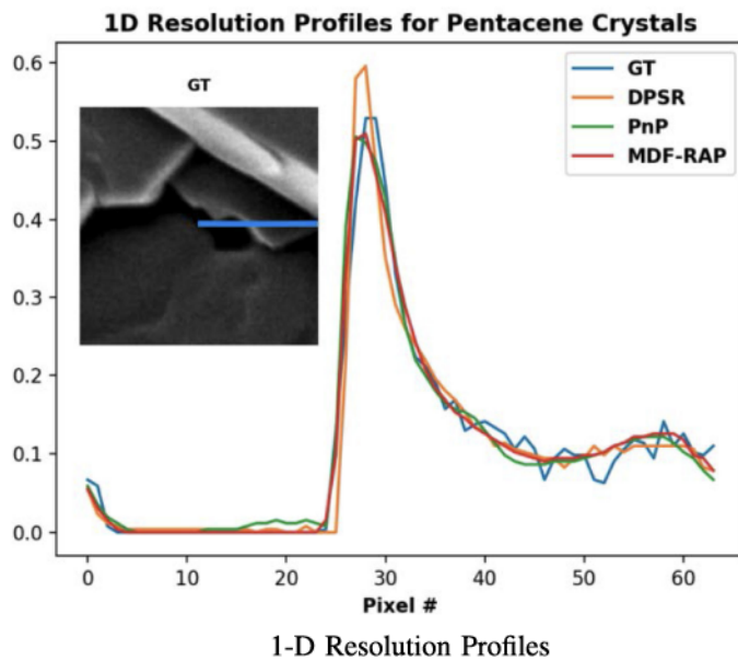
Fig. 6. Left : Plot of intensities along the blue segment for selected reconstructions from Fig. 5. DPSR produces the sharpest edge boundary, while PnP and MDF-RAP better approximate GT image on crystal edges. Right : Comparison of 4x super-resolution reconstructions of a simulated LR EM image of pentacene crystals at varying regularization levels. Note as \mu increases, more detail is present in the final reconstruction. However this can introduce textural artifacts from the forward model into the final reconstruction.
