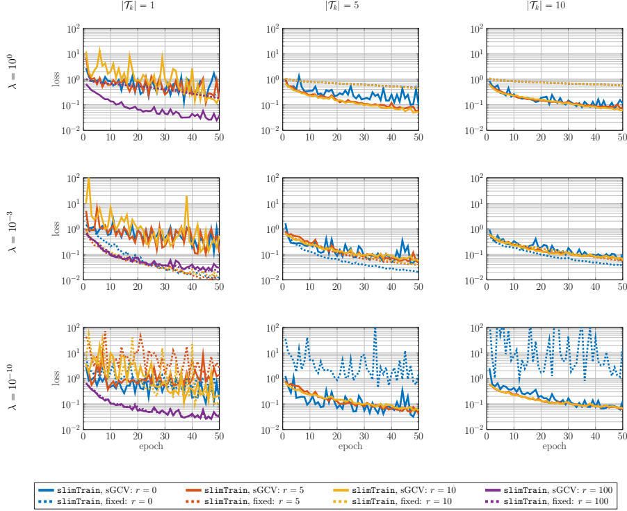
FIG. 2. Convergence of training loss for the peaks experiment when training with slimTrain with a learning rate of \gamma = 10^{-3} . Each row corresponds to a different choice of fixed regularization parameter for \mathbf{W} , \lambda = 10^0, 10^{-3}, 10^{-10} . When training with adaptive regularization parameter selection, the initial regularization parameter \Lambda_0 is set to be the same as the fixed regularization parameter. Each column corresponds to a different batch size, |\mathcal{T}_k| = 1, 5, 10 . Each convergence plot consists of dashed and solid lines corresponding using a fixed regularization parameter and adaptively choosing the regularization parameter using sGCV, respectively. The color of each line corresponds to memory depth r = 0, 5, 10 and, additionally, r = 100 for |\mathcal{T}_k| = 1 .
