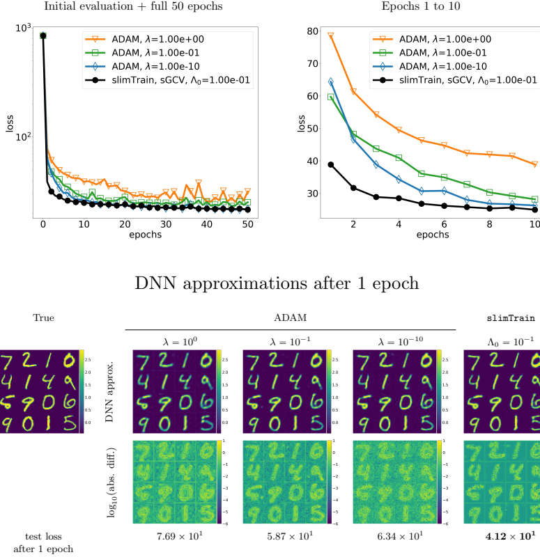
FIG. 8. Training loss convergence and visualizations of MNIST autoencoder approximations. For the convergence plots, the networks are trained for 50 epochs and with recommended learning rate of \gamma = 10^{-3} , batch size of |\mathcal{T}_k| = 32 , regularization parameter \alpha = 10^{-10} for \theta , and 50,000 training images plus 10,000 for validation. For ADAM, we train with three different regularization parameters for \mathbf{w} , \lambda = 10^0, 10^{-1}, 10^{-10} . When using slimTrain , we automatically select the regularization parameters using sGCV with initial parameter \Lambda_0 = 10^{-1} and choose a modest memory depth of r = 5 . We display the DNN approximations after the first epoch below the convergence plots. The top row of MNIST images are, from left to right, 16 test images, the approximation from the ADAM-trained networks with various regularization parameters on \mathbf{w} , and the approximation obtained from slimTrain . The bottom row of images are the absolute differences (in log scale) between the network approximations and the true test images. The value below the absolute difference images is the test loss over all 10,000 test images after the first epoch.
