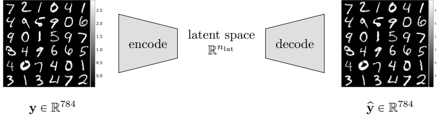
FIG. 7. Illustration of autoencoder for the MNIST data. The goal is to represent high-dimensional data in a low-dimensional, latent space for dimensionality reduction and feature extraction [23]. The encoder is a neural network that maps input data \mathbf{y} to the latent space with intrinsic dimension n_{\text{lat}} (typically user-defined). The decoder is a neural network that maps from the latent space to obtain an approximation of the original input, \hat{\mathbf{y}} .
