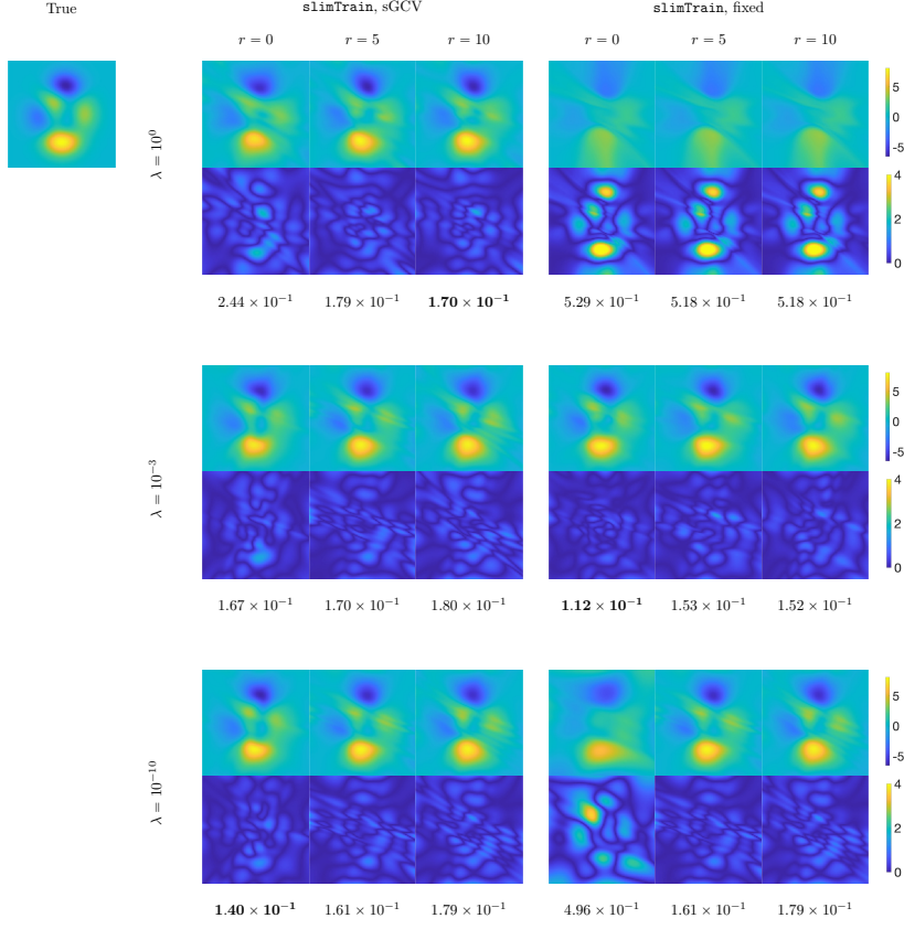
FIG. 3. DNN approximations for the peaks experiment with batch size of |\mathcal{T}_k| = 5 and a learning rate of \gamma = 10^{-3} . The results use the network weights corresponding to the lowest validation loss for each training method. Each block row corresponds to a different choice of fixed regularization parameter for \mathbf{W} , \lambda = 10^0, 10^{-3}, 10^{-10} . The top rows of images in each block depict the DNN approximations of the peaks function. The bottom rows of images in each block depict the absolute difference of the DNN approximations and the true peaks function. The DNN weights used provided the smallest validation loss during training. The relative error of the DNN approximation versus the true function is displayed below the corresponding absolute difference image.
