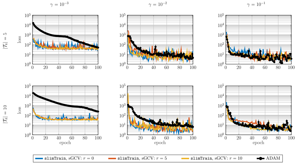
FIG. 5. Convergence results for the training loss for the CDR experiment. The rows correspond to different batch sizes, |\mathcal{T}_k| = 5, 10 , and the columns correspond to different learning rates, \gamma = 10^{-3}, 10^{-2}, 10^{-1} . The colorful, solid lines depict the convergence of the training loss using slimTrain with sGCV regularization parameter selection. Each color corresponds to a different memory depth, r = 0, 5, 10 . The black line with markers depicts the convergence of the training loss using ADAM .
