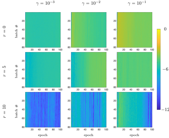
FIG. 6. Effect of learning rate and memory depth on the choice of regularization parameters in the CDR experiment. The presented plots are from training using slimTrain for a batch size of |\mathcal{T}_k| = 5 . We show the regularization parameters (in log scale) obtained for various learning rates (columns) and memory depths (rows).
