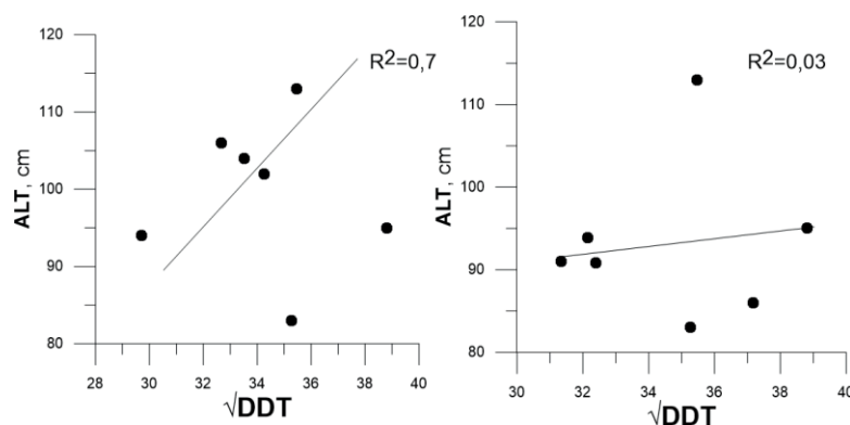
Fig. 5. Dependence of ALT on positive values of air temperature in (a) relatively dry and (b) more humid summer periods
