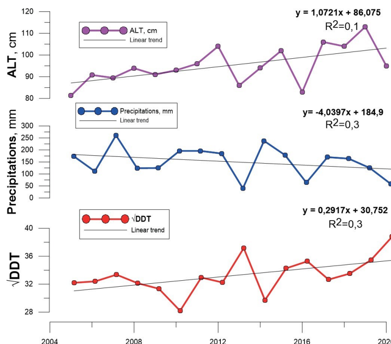
Fig. 3. Time series of active layer thickness, degree days of thawing, and precipitation for the 2005–2020 period
