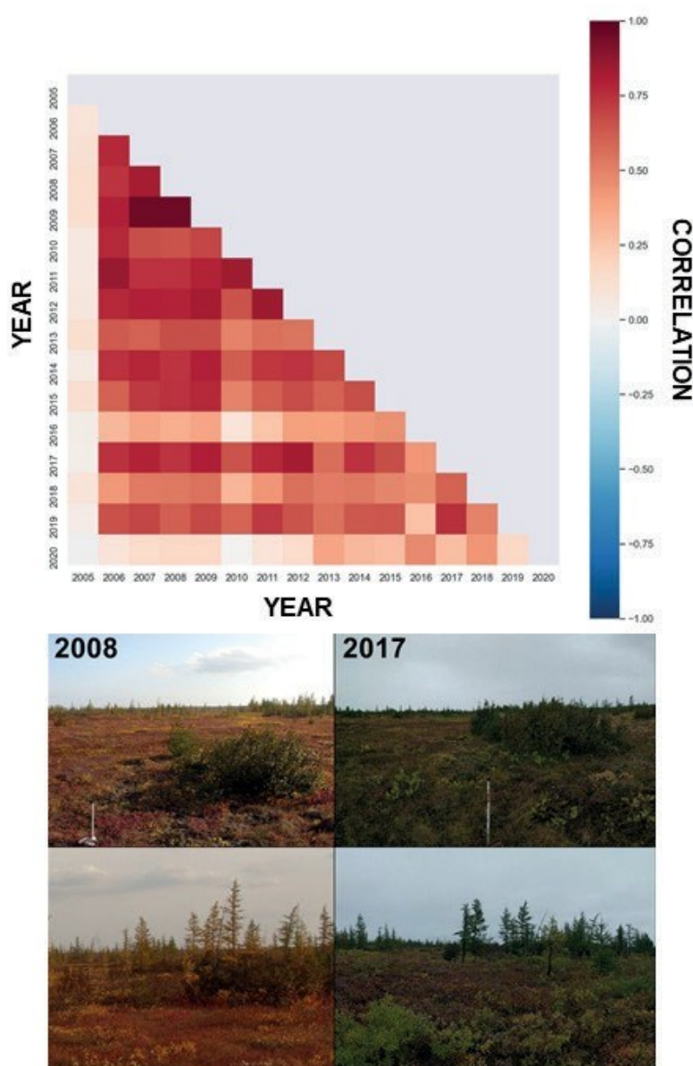
Fig. 9. Results from correlation analysis between the series of active layer thickness data (121 points) for different years. Each cell of the matrix represents the correlation value between two datasets from different years. The bottom part of the figure shows the expansion of bushes at the site. Photos are taken the first point and from the middle of the grid for the period 2008–2017
