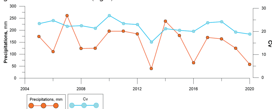
Fig. 6. Graph of the coefficient of variation (standard deviation of indicators for all points from the average value for a particular year) and the amount of summer precipitation
