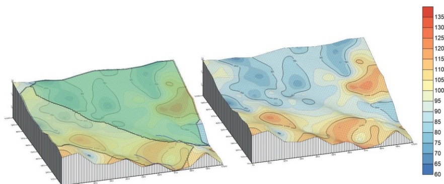
Fig. 8. The microrelief of the site R – 32 with (a) potential water tracks and (b) the average ALT map (2005–2020)
