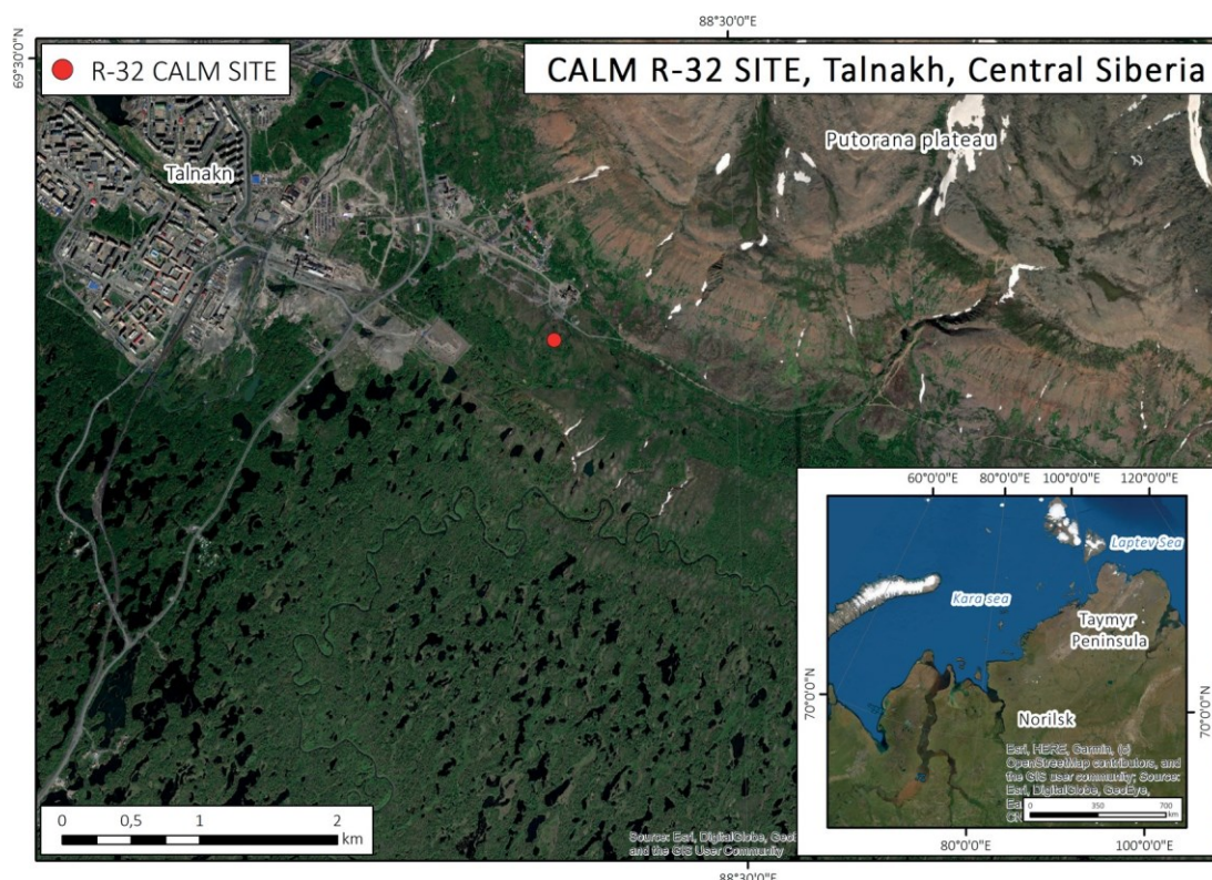
Fig. 1. Location of the R-32 site
