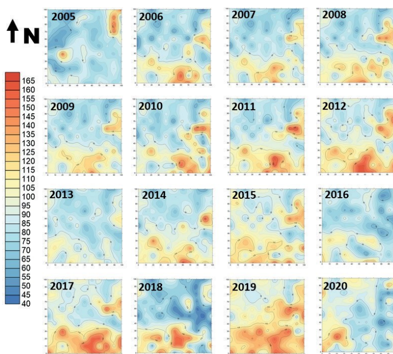
Fig. 7. Active layer thickness maps from 2005 to 2020
