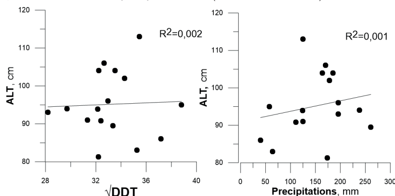
Fig. 4. Dependence of thawing depth on two main factors: the root of positive degree days (a) and summer precipitation (b)
