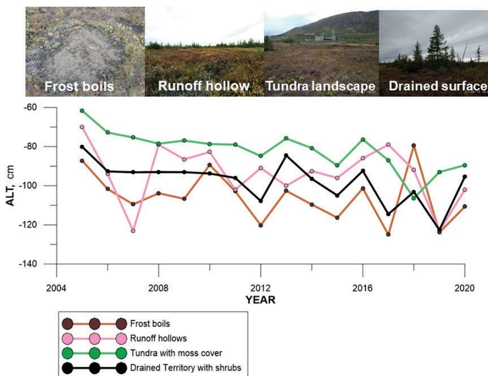
Fig. 11. Active layer thicknesses in different landscape types
