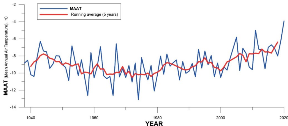
Fig. 2. Changes in mean annual air temperature in Noril'sk (data from the Noril'sk Meteorological Observatory). Blue line represents mean annual air temperature (MAAT). Red line represents the 5-year running average
