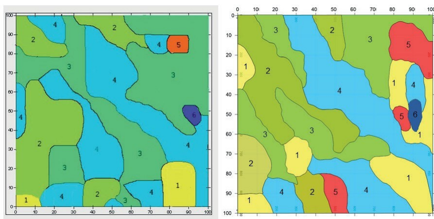
Fig. 10. Active layer thickness maps from 2005 to 2020
