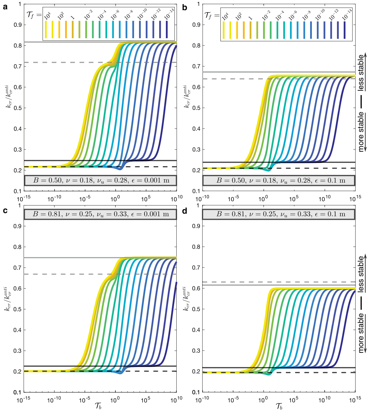
Figure 3. Changes in critical wavenumber k_{cr} , non-dimensionalized by k_{cr}^{anti} , when varying \tau_b but keeping \tau_f fixed, for in-plane shear. Definitions of lines and panels are the same as in Figure 2.
