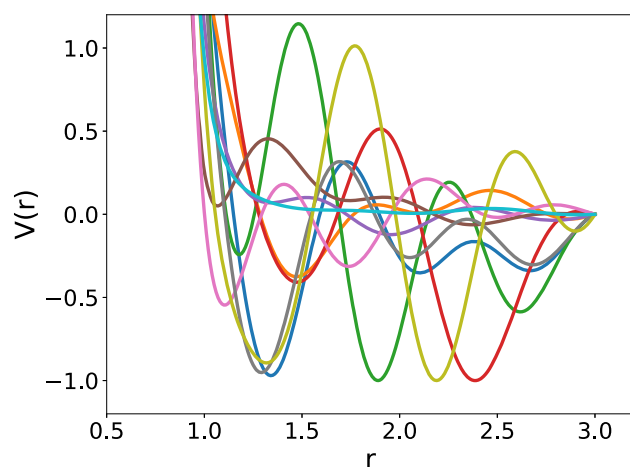
Fig. 3 Initial potentials used for digital alchemy simulations
