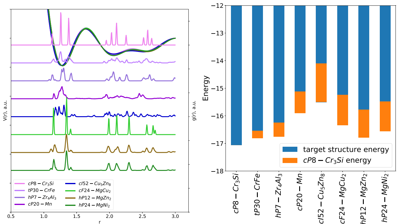
Fig. 6 Eight structures in the same similarity group that yield very similar cP8-Cr_3Si -forming potentials. Left: RDFs and optimized pair potentials using Alch-MD for each structure. Right: Comparison of their potential energies
