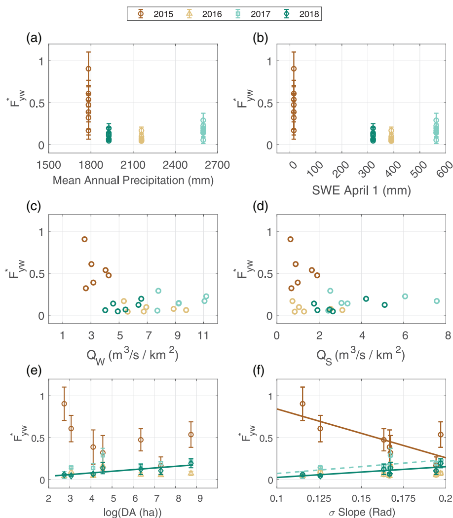
FIGURE 7 Relationship between young water fraction ( F_{yw}^* ) and (a) Mean annual precipitation, (b) April 1st snow water equivalent (SWE), (c) Mean daily winter discharge, (d) Mean daily spring discharge, (e) Drainage area (DA), and (f) SD of water slope ( \sigma slope). A solid line indicates a relationship with a p -value < 0.05 and a dash line indicates a relationship with a p -values between 0.05 and 0.1
