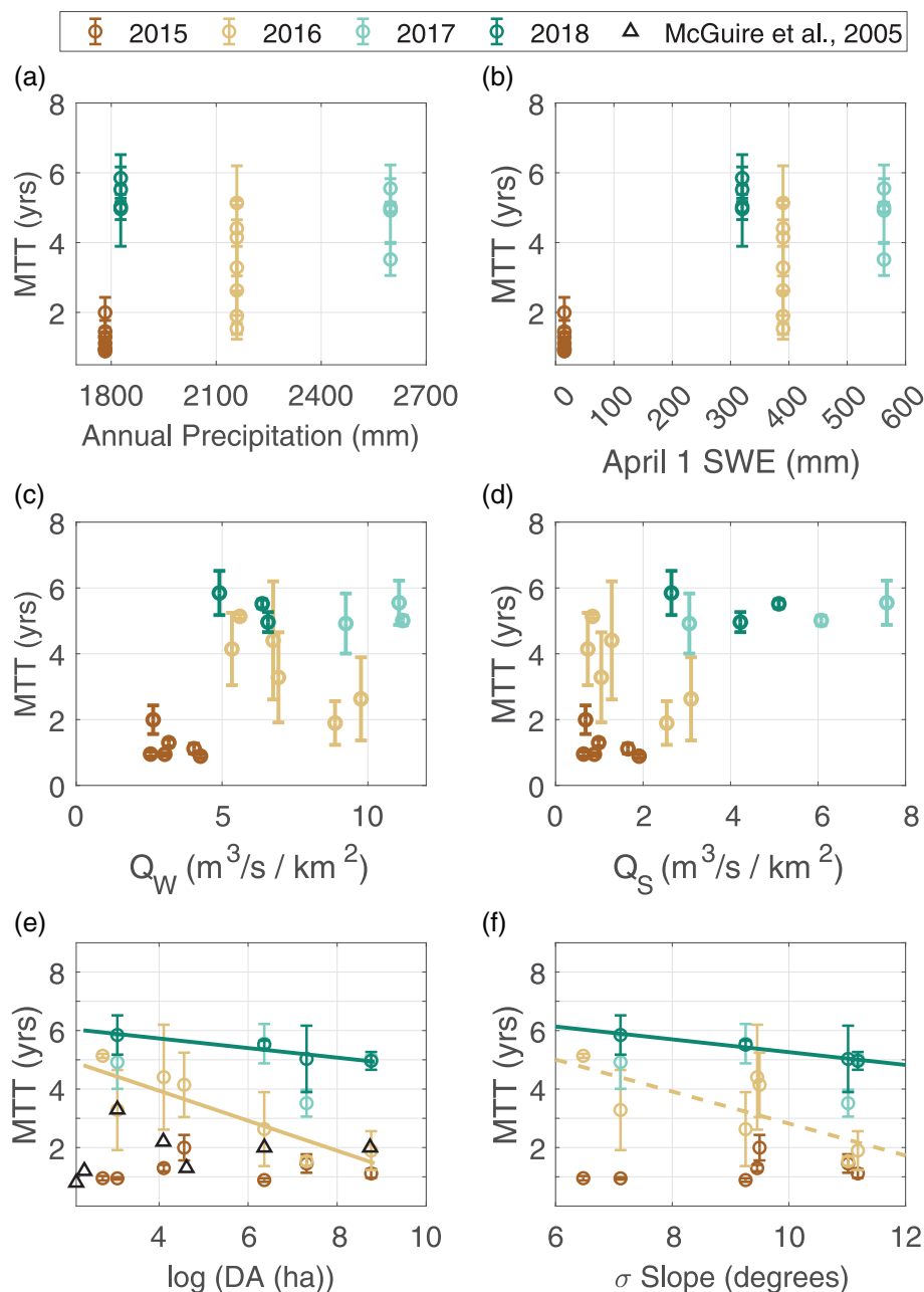
FIGURE 6 Relationship between mean transit time (MTT) and (a) Mean annual precipitation, (b) April 1st snow water equivalent (SWE), (c) Mean daily winter discharge, (d) Mean daily spring discharge, (e) Drainage area (DA), and (f) SD of water slope ( \sigma slope). A solid line indicates a relationship with a p -value <0.05 and a dash line indicates a relationship with a p -values between 0.05 and 0.1
