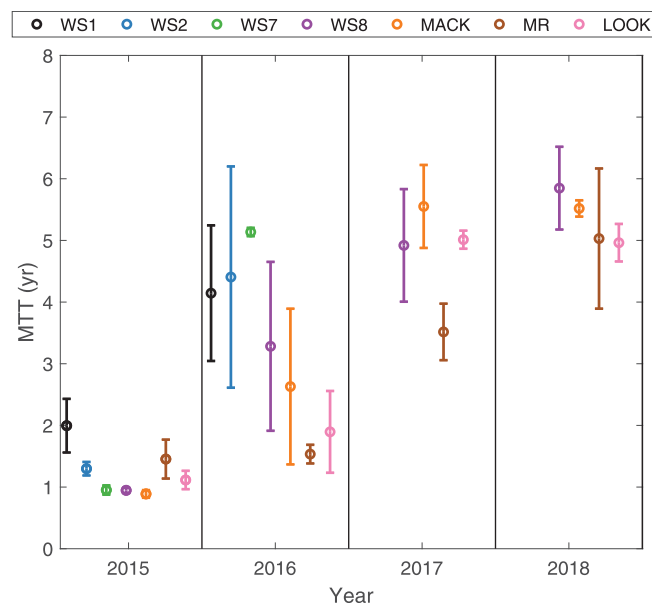
FIGURE 5 Mean annual MTT for seven watersheds in the Andrews Forest (Figure 1). Each point and bar represent the mean and SD of the MTT estimated across 13–14 2-year windows spaced every 2 weeks around the year of interest (Table 3)
