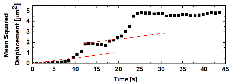
FIGURE 5. Mean squared displacement of the microgel tracked in Fig. 4b (the dashed lines correspond to the expected time dependence of the mean squared displacement for an assembly of thermally diffusing particles).
