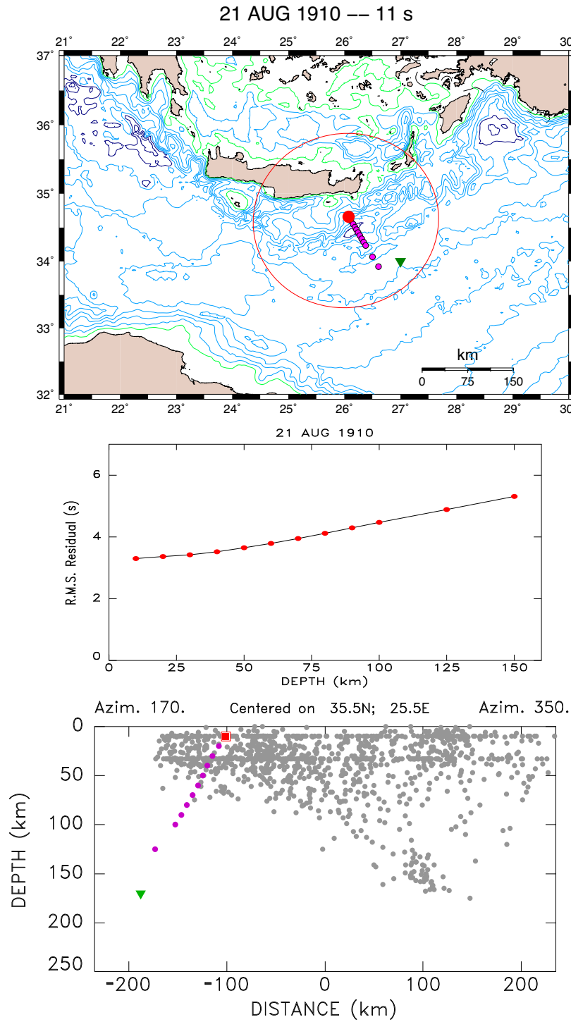
Figure A5. Relocation of the 1910 earthquake. All symbols are defined in Appendix B.
