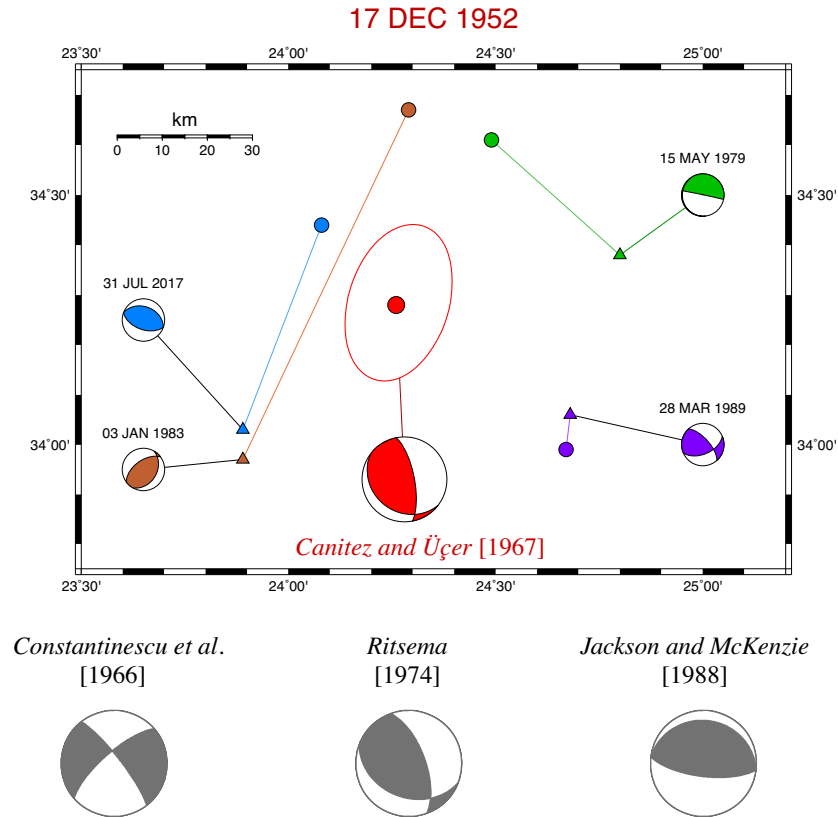
Figure A2. Focal mechanisms of the 1952 earthquake and neighbouring events. The map reproduces our relocation, with associated ellipse, and the preferred mechanism of Canitez & Üçer (1967). The focal mechanisms of the four closest GlobalCMT solutions are also shown; note the large disparity in geometries. For each event, the colour-coded solid dot represents the relocated ISC epicentre, and the triangle the GCMT centroid; note the occasional large distance between them. Alternate focal solutions for the 1952 are also shown in grey below the map.
