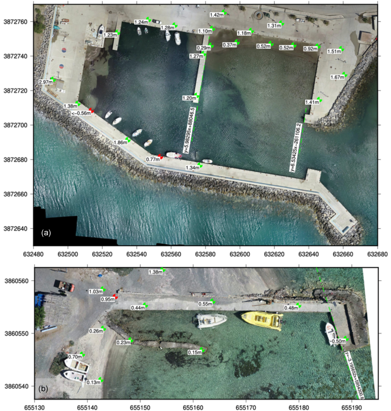
Figure A9. Orthophoto maps of the harbours in (a) Arvi and (b) north Chrsi, produced using drone aerial images. The GCP's used for the orthorectification and the corresponding elevations are shown with the green points. The surveyed runup/drawdown points are shown in red. The lines projected along docks that were used to extract the water level from eyewitness images (Fig. A8) are shown with the green dashed–dotted lines. Grid coordinates correspond to the (projected) Hellenic Geodetic Reference System 1987 (HEMCO 1987; Veis 1996): x -axis corresponds to the Easting (m) and the y -axis to the Northing (m).
