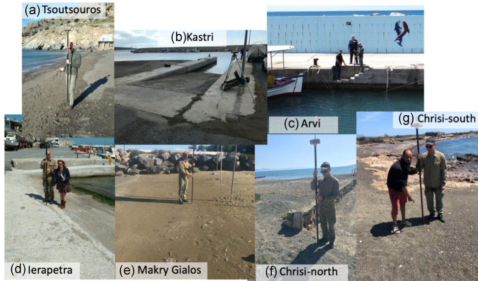
Figure A7. Pictures of tsunami runup data collected in seven coastal locations.
