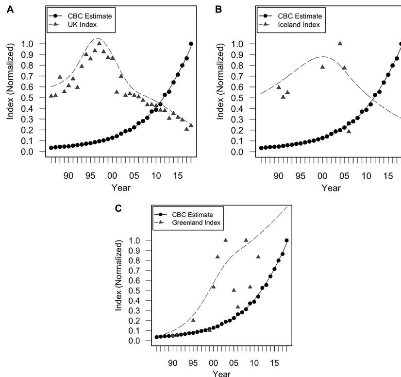
FIGURE 4 | Indices of annual breeding population size from 1986 to 2018 for (A) the UK, (B) Iceland (colony of Midnesheidi), and (C) Greenland (colony of Eqauiut), and Christmas Bird Count (CBC) trend estimates of vagrants. Trend estimates are calculated from CBC surveys as estimates of median abundance, using Bayesian hierarchical methods (Soykan et al., 2016; Meehan et al., 2020). Normalized values were obtained by dividing each value in a given dataset by the maximum value of that dataset.
