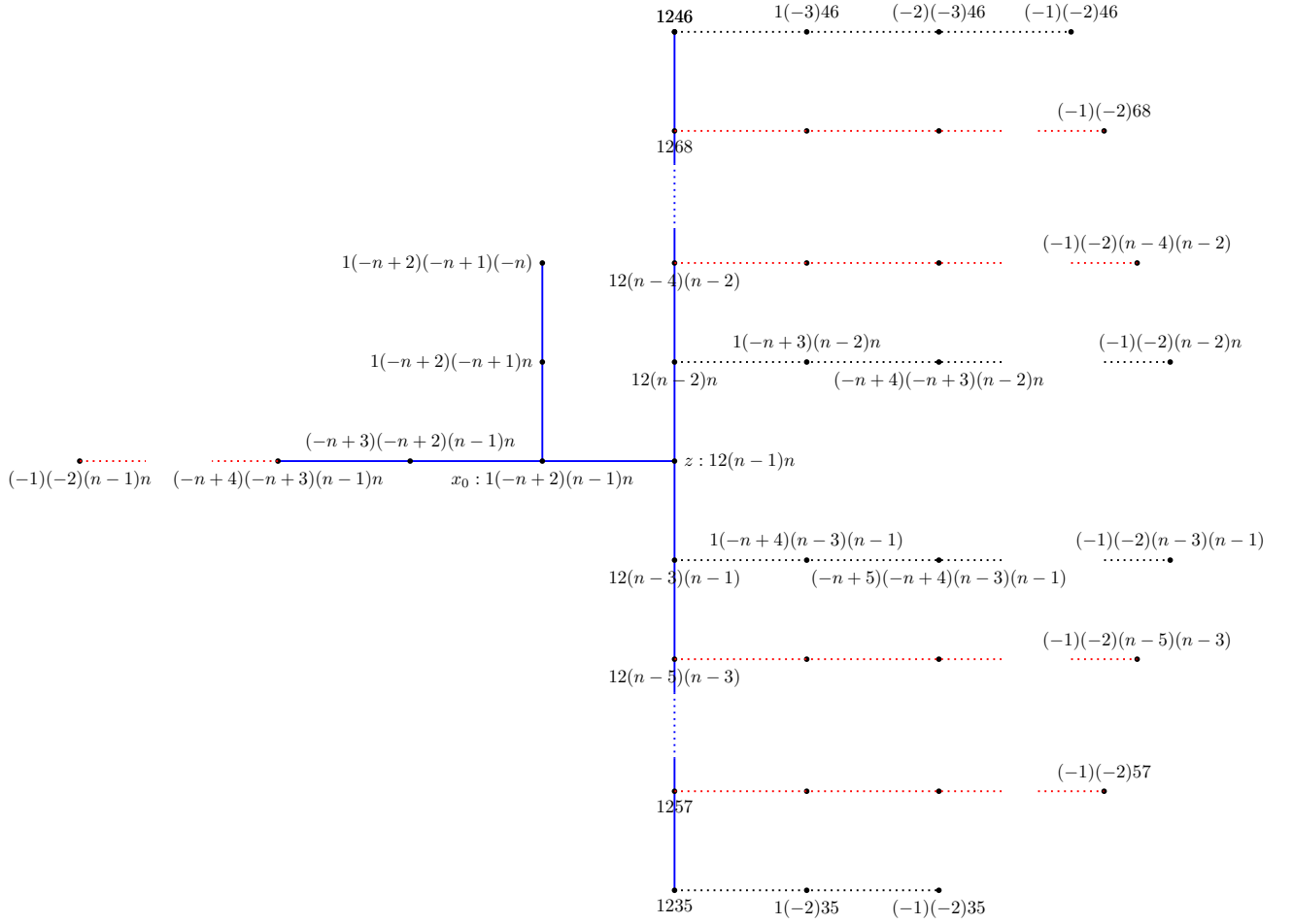
Figure 1: A subgraph of the facet-ridge graph of \Delta_n^3 when n is even
