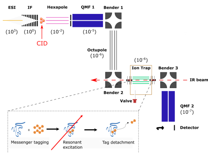
Figure 2: Schematic representation of the experimental setup to obtain IR spectra of mass selected CID fragments under cryogenic conditions. Pressures, in mbar, are indicated in brackets for each differentially pumped section. The bottom left inset illustrates the principle of messenger tagging spectroscopy.
