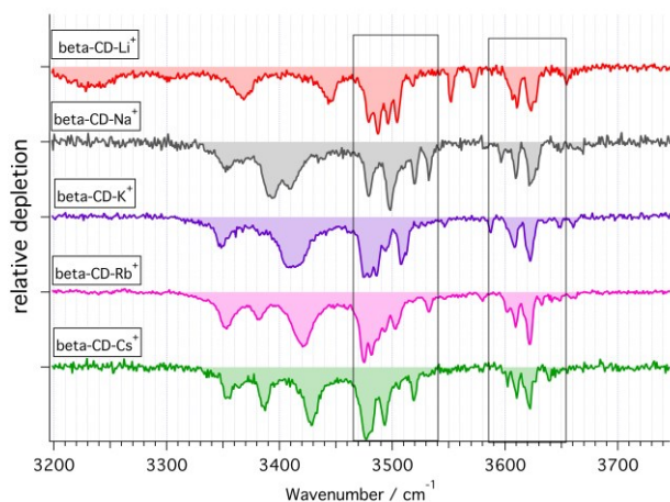
Figure 5: Cryogenic IR spectra of \beta -CD complexed with group I cations. The two marked areas denote the transitions associated to the C2 and C3 OH oscillators.
