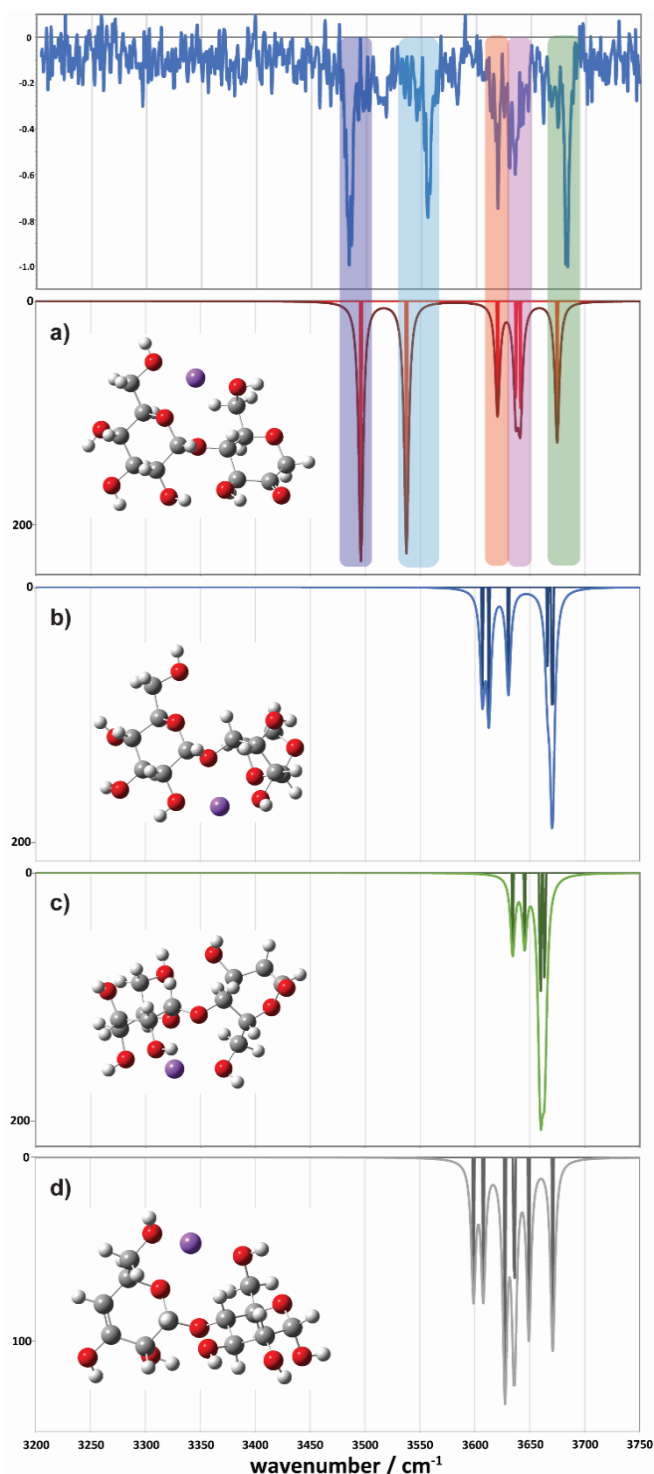
Figure 7: Comparison between the experimental (top) and simulated IR spectra for the m/z 347 fragment. (a) represents the ketone, (b) the 1-6 anhydro, (c) the 1-2 anhydro and (d) the Z fragment structures.
