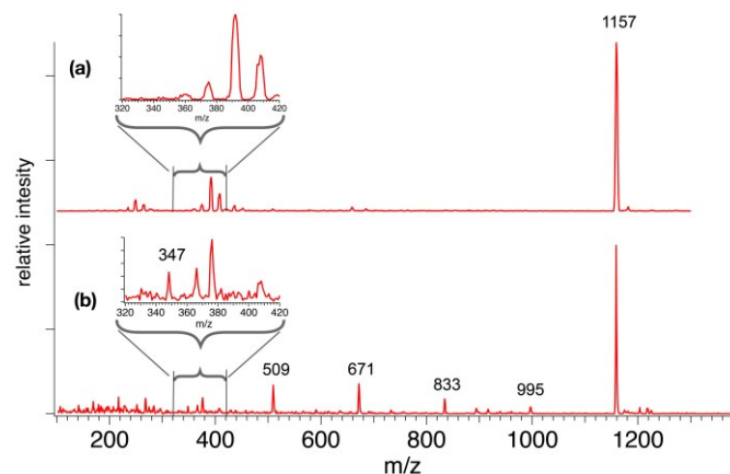
Figure 3: CID-MS of sodiated \beta -CD and its fragments, carried out with a potential difference of 100 V (a) and 240 V (b) in our tandem mass spectrometer. Consecutive loss of 162 m/z is observed from the parent at 240 V, while no fragments are observed at 100 V.
