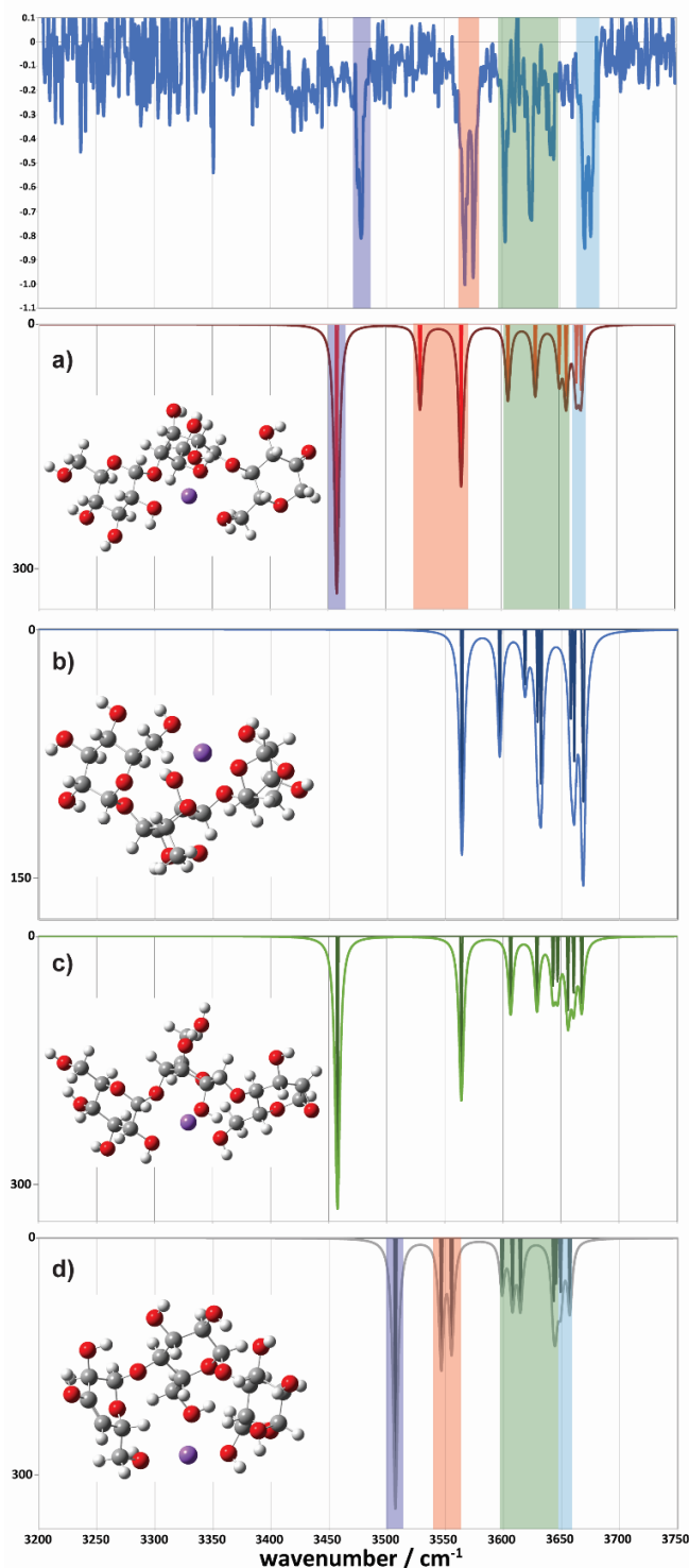
Figure 8: Comparison between the experimental (top) and simulated IR spectra for the m/z 509 fragment. (a) represents the ketone, (b) the 1-6 anhydro, (c) the 1-2 anhydro B_3 and (d) the Z_3 fragment structures.
