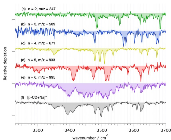
Figure 6: Cryogenic IR spectra of the main CID fragments of [\beta\text{-CD+Na}]^+ (a-e) and the parent ion (f). The index n refers to the number of monosaccharides in each fragment.
