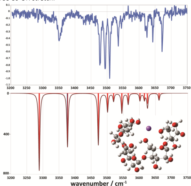
Figure 9: Comparison between the experimental (top) and simulated IR spectra for the m/z 671 fragment. The simulated spectrum represents a 2-ketone B_4 structure at 7.9 \text{kJ/mol} .
