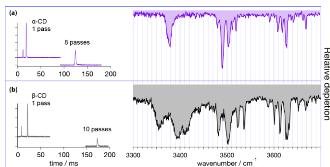
Figure 4: Arrival times of [\alpha\text{-CD}+\text{Na}]^+ (a) and [\beta\text{-CD}+\text{Na}]^+ (b) and their corresponding cryogenic IR spectra. Note that the fast ATD peak in the left panels of (a) and (b) corresponds to doubly charged dimers of the corresponding cyclodextrins that cannot be discriminated by our quadrupole mass filter and are propelled faster through the IMS buffer gas due to their doubly charged character.
