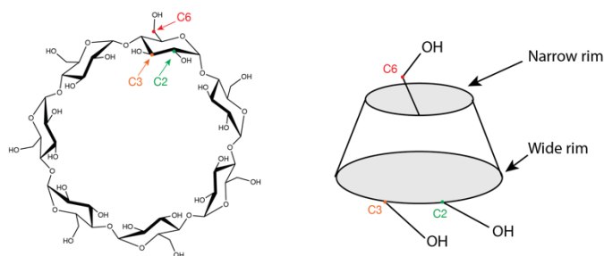
Figure 1: Schematic representation of \beta -cyclodextrin, with its conical structure represented on the right. The carbon atoms connected to the hydroxyls are labelled C2, C3 and C6 for one glucose unit.
