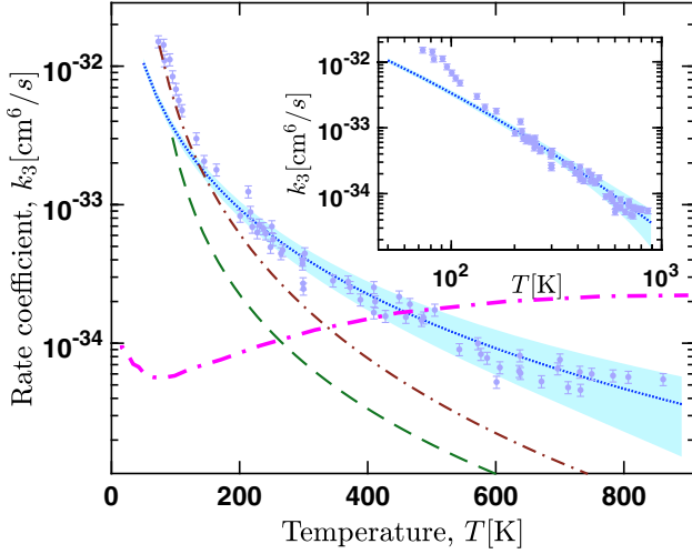
FIG. 4. Thermally averaged recombination rate coefficients for formation of molecules with all binding energies scaled by the factor of 50 \text{ cm}^{-1}/T accounting for the process of vibrational quenching (solid line). The shaded area (light blue) represents the uncertainty of the theoretical model. The circles with error bars are the same experimental data as in Fig. 3. Previous theoretical results are shown with a thick dash-dotted (magenta) line [30], thin dash-dotted (brown) line [9], and dashed (green) line [28]. The inset shows the data in the log-log scale.
