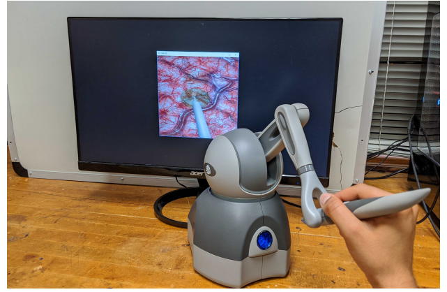
Fig. 7: The typical experimental setup. The user interacts with the simulation both visually and haptically through a stylus haptic device, through which motion commands are sent and force feedback is received.
