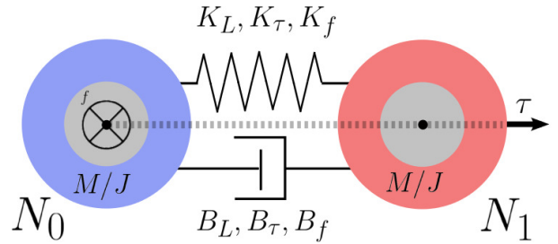
Fig. 3: Translational and rotational physical elements that govern node-to-node ( N_0 and N_1 are nodes) dynamic interaction. M, J are translational and rotational inertias, and K_L, K_\tau, K_f and B_L, B_\tau, B_f are linear spring and damping coefficients for translation, torsion and flexion respectively.
