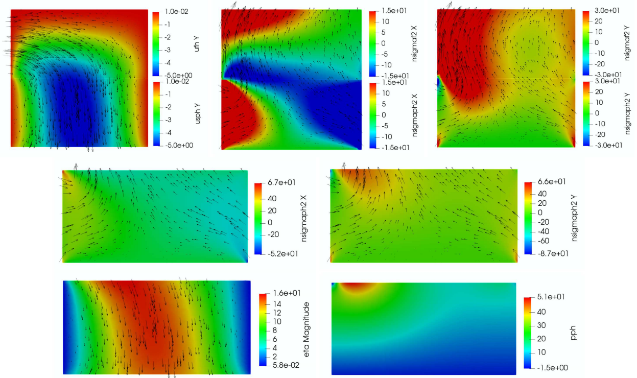
FIGURE 2. Example 2, Case 2, \mathbf{K} = 10^{-4} \times \mathbf{I} , s_0 = 10^{-4} , \lambda_p = 10^6 , \mu_p = 1 . Computed solution at final time T = 3 . Top left: velocities \mathbf{u}_f and \mathbf{u}_p + \partial_t \boldsymbol{\eta}_p (arrows), u_{f,2} and u_{p,2} + \partial_t \eta_{p,2} (color). Top middle and right: stresses -(\sigma_{f,12}, \sigma_{f,22})^t and -(\sigma_{p,12}, \sigma_{p,22})^t (arrows); top middle: -\sigma_{f,12} and -\sigma_{p,12} (color); top right: -\sigma_{f,22} and -\sigma_{p,22} (color). Middle: poroelastic stress -(\sigma_{p,12}, \sigma_{p,22})^t (arrows); middle left: -\sigma_{p,12} (color); middle right: -\sigma_{p,22} (color). Bottom left: displacement \boldsymbol{\eta}_p (arrows), |\boldsymbol{\eta}_p| (color). Bottom right: Darcy pressure p_p .
