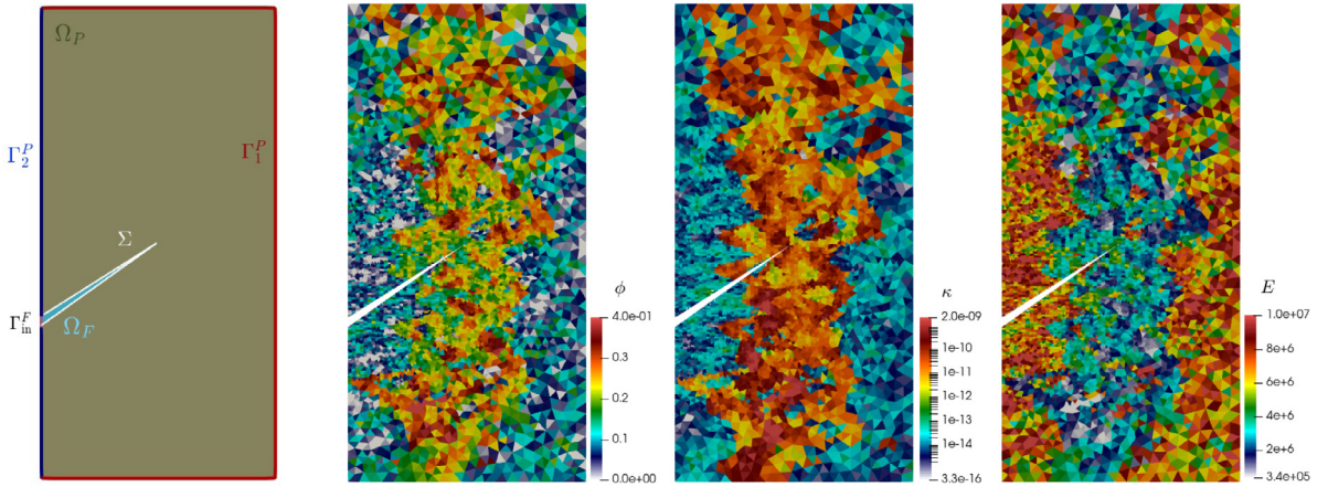
Fig. 6.3. Example 3. Schematic representation of sub-domains, location of the free-porous interface, and configuration of sub-boundaries (left panel); and material properties (porosity \phi(\mathbf{x}) , permeability \kappa(\mathbf{x}) , and Young modulus E(\mathbf{x}) ) from layer 80 of the SPE10 benchmark dataset for reservoir simulations, herein projected onto a coarse mesh for the poroelastic sub-domain.
