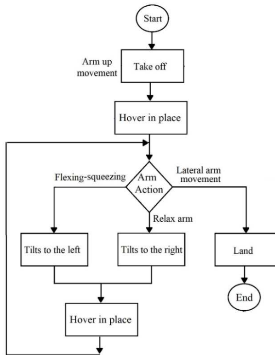
Fig. 4 Flowchart of the drone commands
