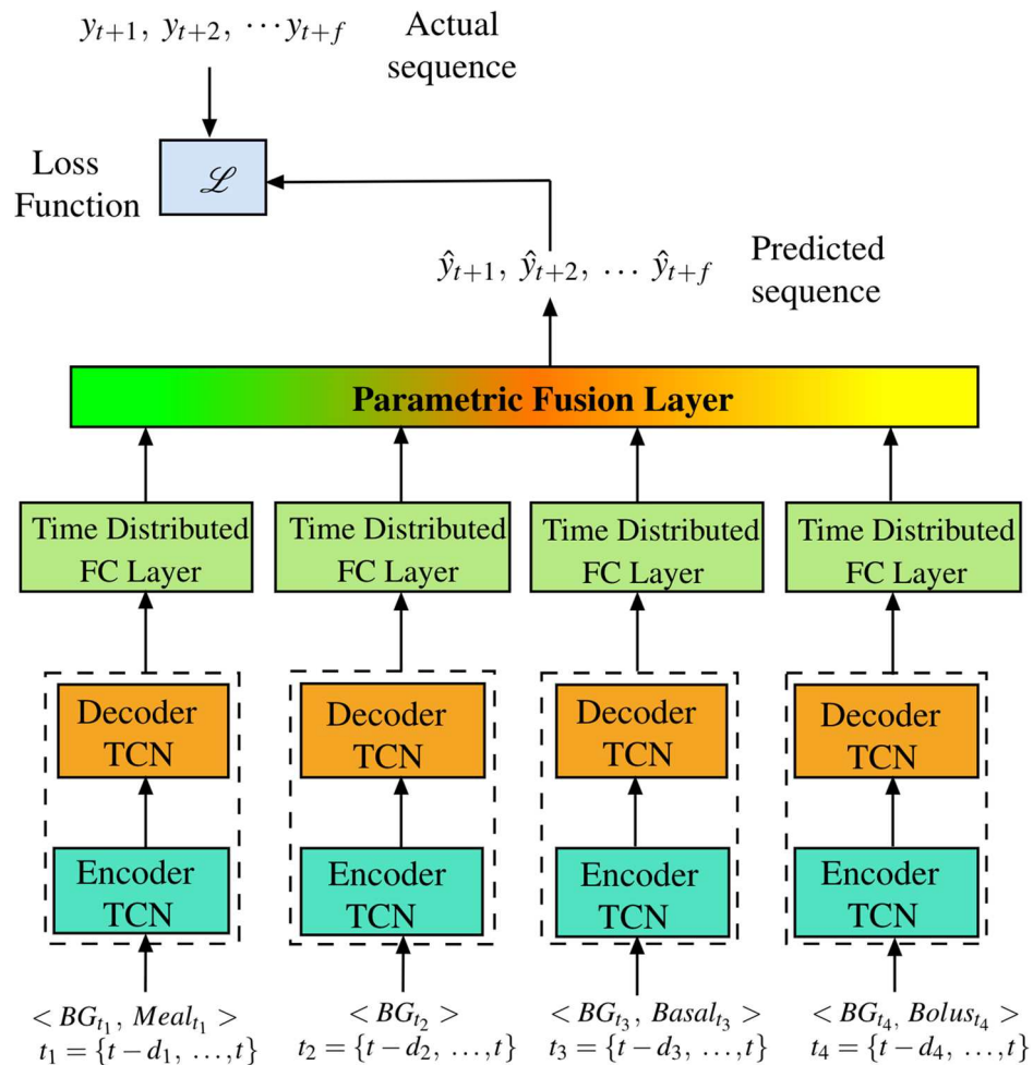
Figure 6. Proposed model.
