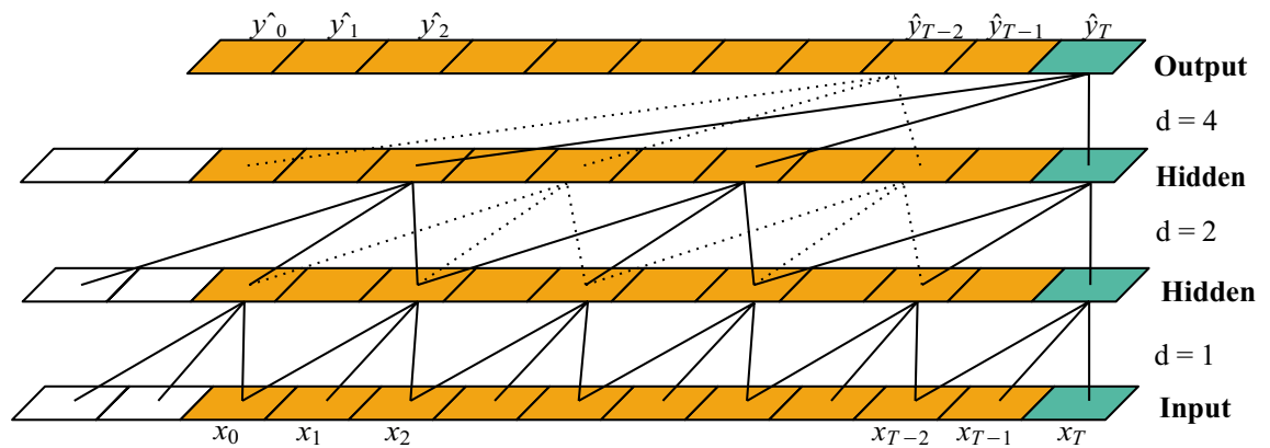
Figure 3. Dilated causal convolutions with dilation factor d = 1, 2, 4 , and kernel size, k = 3 .
