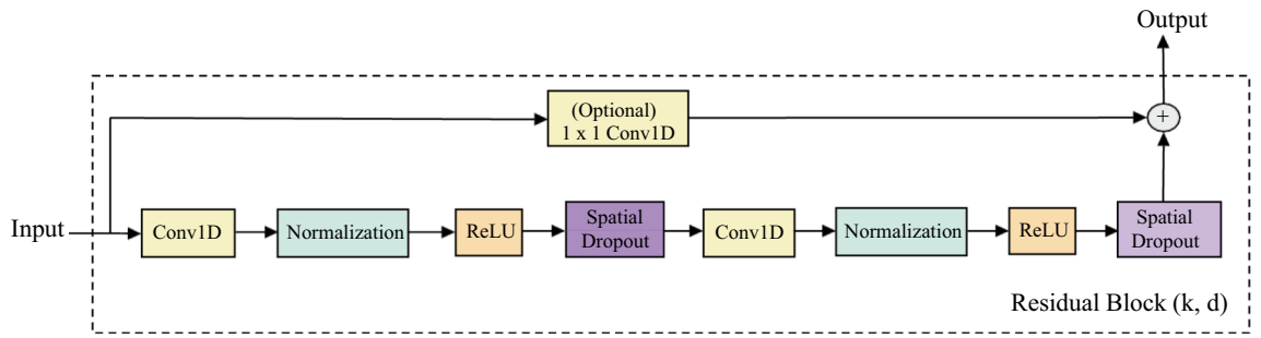
Figure 4. Residual block in temporal convolutional network.
