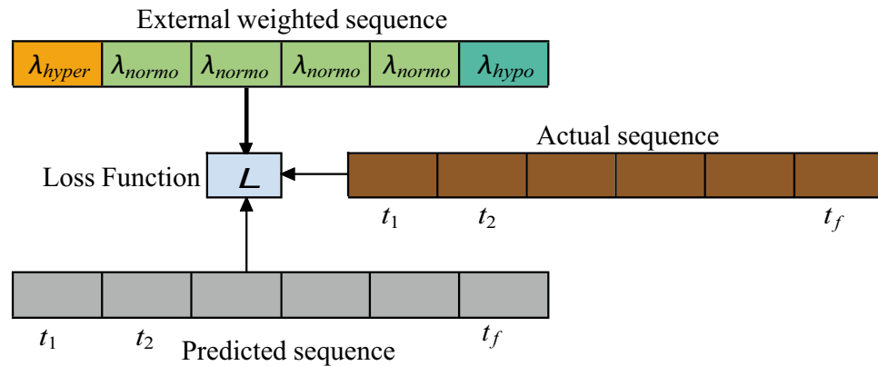
Figure 7. Weighted loss function.
