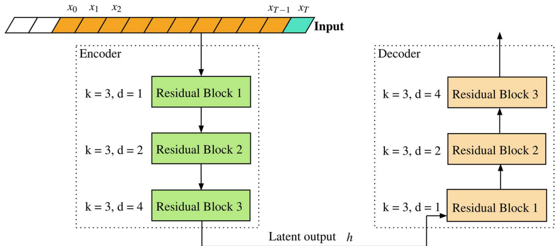
Figure 5. Sequence-to-sequence approach.
