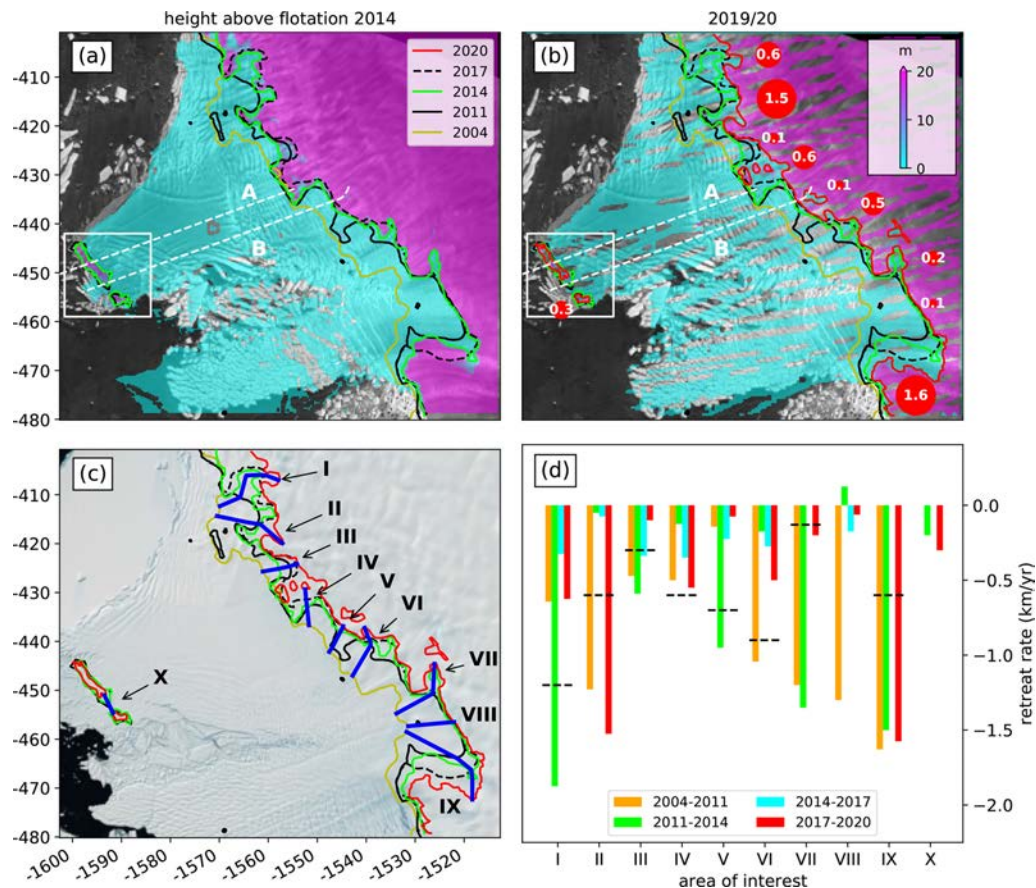
Figure 3. Regional changes: height above flotation from (a) REMA data in 2014 and (b) ICESat-2 surface altimetry data in 2019/20 overlain on a Sentinel 1 SAR image from October 2019. Airborne surveys from 2009 and 2019 (a, b) are shown as dashed white lines. Red circles in panel (b) show rates of grounding-line retreat since the last assessment in 2017 (Milillo et al., 2019). Roman numerals in panel (c) refer to areas of interest discussed in the text and are overlain on the Landsat Image Mosaic of Antarctica (Bindschadler et al., 2008). Panel (d) shows histograms of grounding-line retreat rates along the (blue) profiles in panel (c) in comparison to (dashed black) the InSAR-derived retreat rates between 2011 to 2017 from Milillo et al. (2019). The white rectangle (a, b) shows the spatial extent of Fig. 5.
