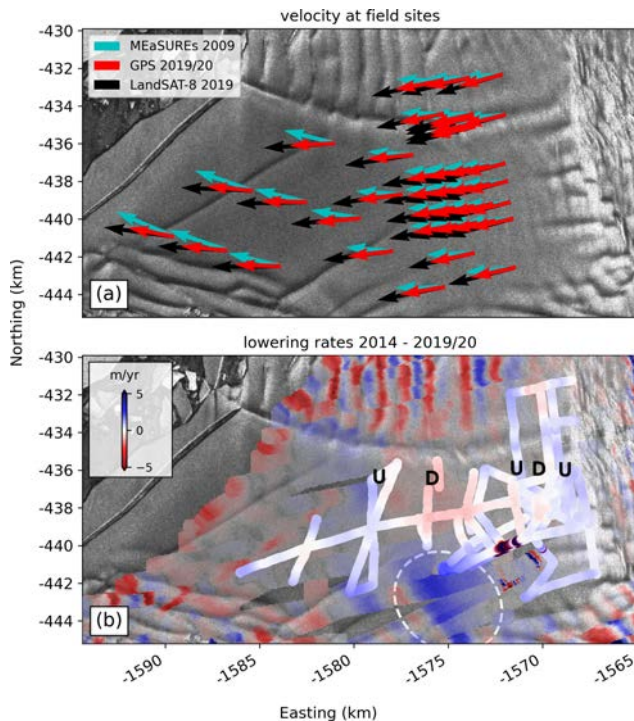
Figure 6. Validation of remote-sensing observations with static and kinematic GPS measurements on the Eastern Ice Shelf overlain on a Sentinel 1 SAR image from October 2019: (a) Counterclockwise rotation of ice flow between 2009 from MEaSUREs to 2019 from Landsat-8 feature tracking in comparison with results from a recent GPS repeat survey. The black Landsat-8 vectors have been lengthened by 33 % to increase visibility under the red GPS vectors and are in excellent agreement with the measurements. (b) Comparison between recent Lagrangian rates of surface lowering from a kinematic GPS survey to validate Lagrangian surface-lowering rates derived from ICESat-2 data. Positive values indicate thickening, while negative-value areas delineate vertical thinning. White colors were coded transparent in the ICESat-2 data to highlight the GPS tracks. Tracks were plotted at their migrated locations in 2014. The letters U and D indicate areas of local hydrostatic imbalance, where the ice surface is going up and down, respectively. The dashed white oval shows the location of a spurious thickening signal that we interpret as an artifact from feathering between individual REMA strips.
