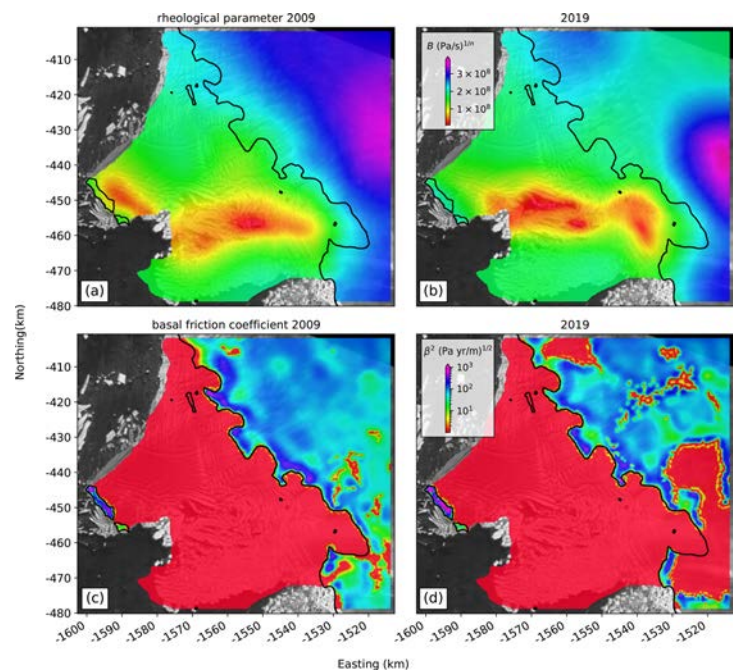
Figure A2. Inferred fields of the rheological parameter and the basal friction coefficient from the iterative inversion using both the MEaSUREs and our Landsat-8 velocity field. Note (i) the rheological weakening of the shear margin between the Eastern Ice Shelf and the Western Glacier Tongue, (ii) the misrepresented rheological strengthening of the shear zone upstream of the pinning point that is clearly absent in visible satellite imagery, (iii) high values of the basal friction coefficient at the pinning point, and (iv) very low friction values underneath Thwaites Glacier’s main trunk that suggest distributed thawed bed properties.
