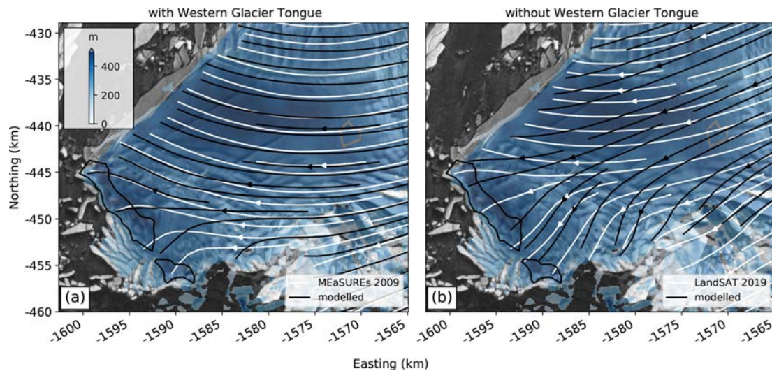
Figure 8. Comparison between (white) satellite-derived streamlines and (black) numerical solutions from ISSM: (a) the situation before the breakup of the Western Glacier Tongue in 2009 with a relatively well-grounded pinning point. (b) Removing the Western Glacier Tongue from the model domain, and thus weakening its influence on the Eastern Ice Shelf, reproduces the flow divergence around the pinning point as observed in the satellite data but overestimates the counterclockwise rotation of ice flow. This suggests that the Eastern Ice Shelf has not yet fully decoupled from the Western Glacier Tongue, particularly closer to the grounding line. Blue colors correspond to the ice thickness estimate derived in this study.
