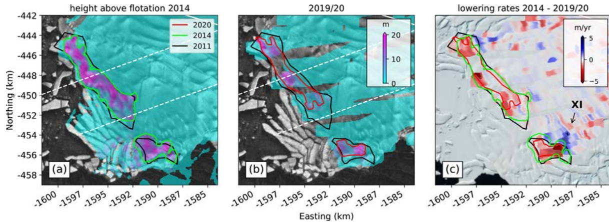
Figure 5. Close-up of the pinning point area and calculated height above flotation (a) from REMA and (b) ICESat-2 data. (c) Lagrangian rates of surface lowering. Red colors indicate thinning, while blue areas delineate thickening. The green and red lines show the reduced extent of the pinning point as estimated from height above flotation in 2014 and 2019/20, respectively. Map background is a Sentinel 1 SAR image from October 2019 and the Landsat Image Mosaic of Antarctica (Bindshadler et al., 2008). The Roman numeral in panel (c) refers to an area of interest discussed in the text.
