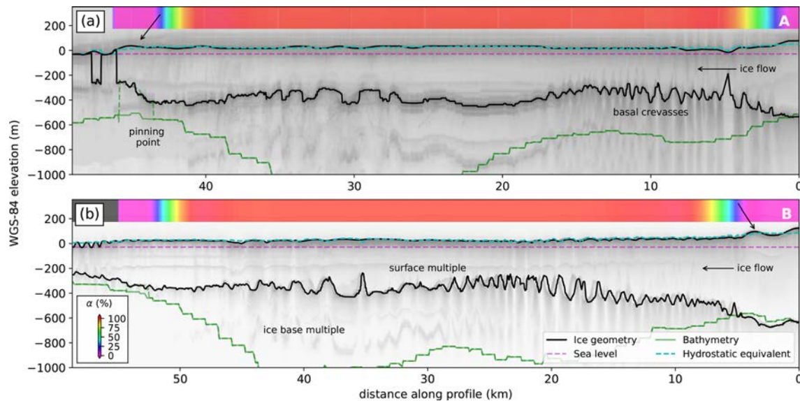
Figure 2. Radargrams from airborne radar surveys (a) in November 2009 and (b) in January 2019 revealing a heavily crevassed ice-base topography. Transects from the grounded ice (right), across the tidal-flexure zone as predicted by an elastic model based on the 2011 grounding line (Rignot et al., 2016) onto large parts of the freely floating ice shelf and (left) ultimately crossing the pinning point that is buttressing the Eastern Ice Shelf. Colors show the percentage tidal displacement with red areas experiencing the full range of the tidal oscillation, while the remaining areas are subject to tidal ice-shelf flexure. Purple areas are grounded according to the 2011 grounding line for the pinning point and the 2017 main grounding line of Thwaites Glacier. The dashed blue line shows flotation height. Grounded areas with surface elevation above flotation height are indicated by black arrows.
