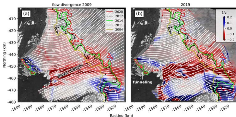
Figure 4. Ice flow divergence from (a) MEaSUREs data in 2009 and (b) Landsat-8 feature tracking in 2019 overlain on a Sentinel 1 SAR image from October 2019. Blue colors denote flow divergence and red colors flow convergence. Note the upstream migration of the shear zone near the pinning point and the funneling of ice streamlines between the two remaining portions of the pinning point.
