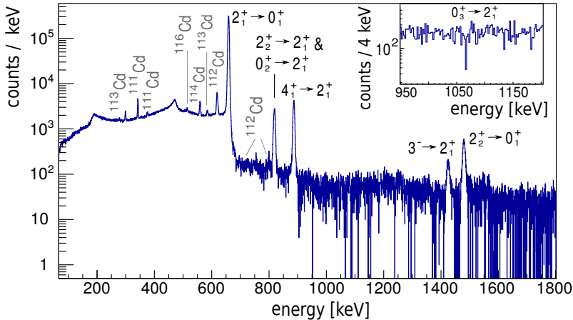
Fig. 1. Doppler-corrected and background subtracted \gamma -ray spectrum of ^{110}\text{Cd} . Gamma-rays from Coulomb excitation of target contaminants, ^{111-114}\text{Cd} and ^{116}\text{Cd} , are also visible. Inset: Part of the same spectrum expanded around the vicinity of the weak 0_3^+ \rightarrow 2_1^+ \gamma -ray transition.
